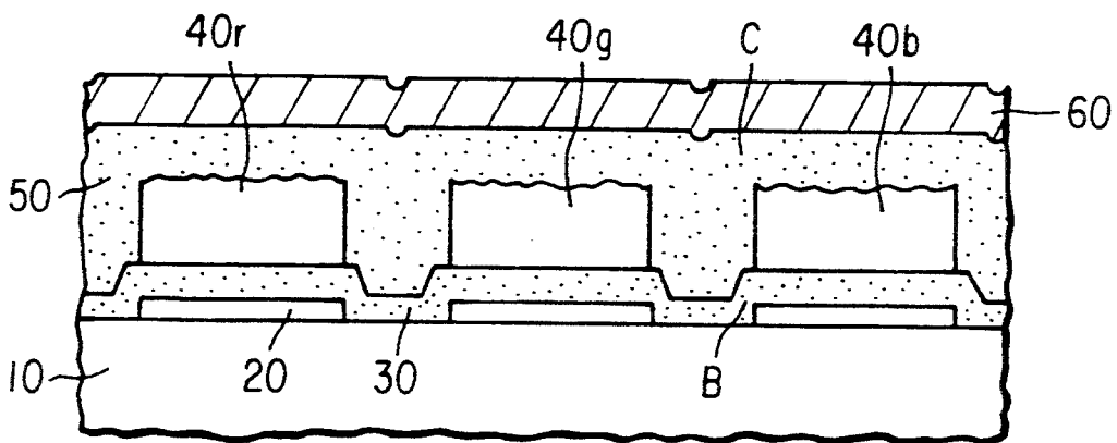
FIG. 7 (prior art)
