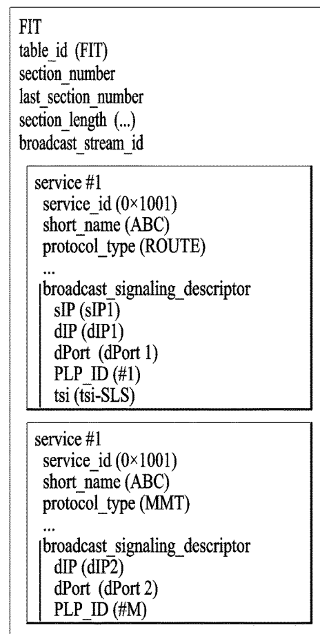
Syntax B
