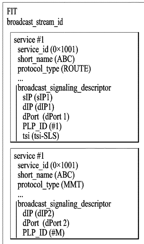
Syntax A
