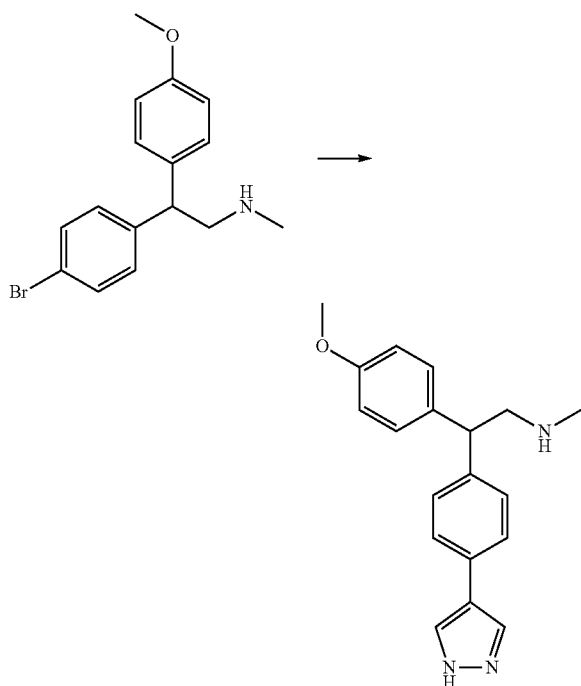
46C. {2-(4-Methoxy-phenyl)-2-[4-(1H-pyrazol-4-yl)-phenyl]-ethyl}-methyl-amine
