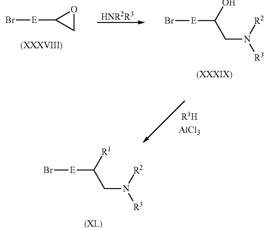
Scheme 4
