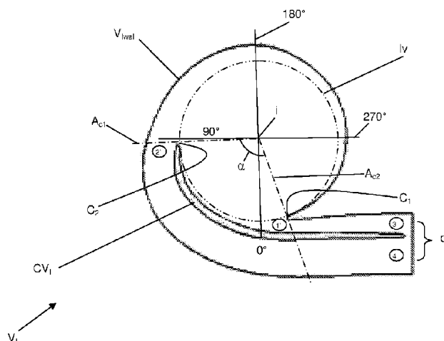
Dual Volute According to the Present Invention
