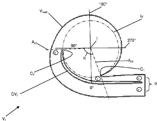
Dual Volute According to the Present Invention
