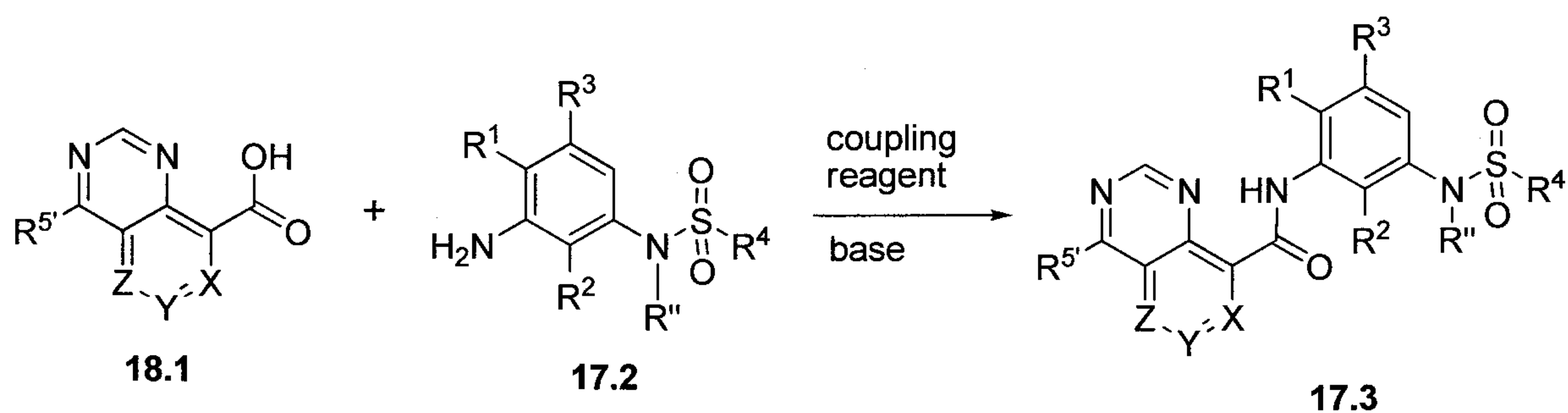
Scheme 18
