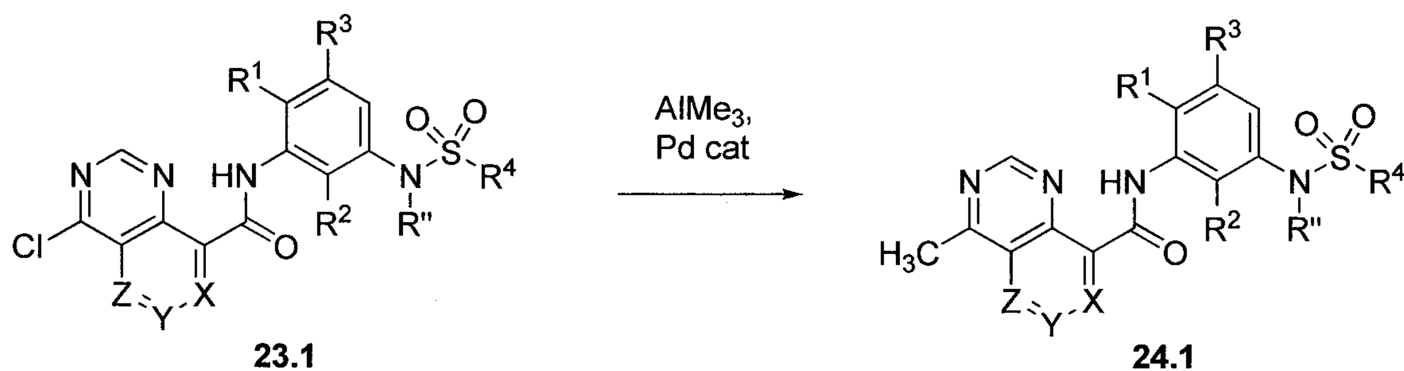
Scheme 24
