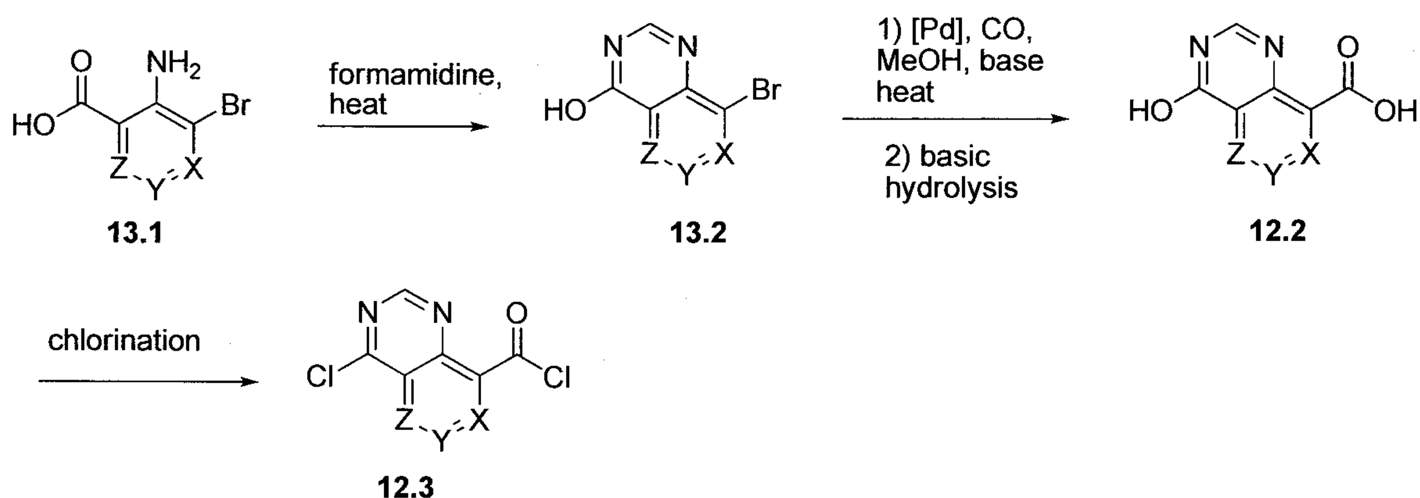
Scheme 13
