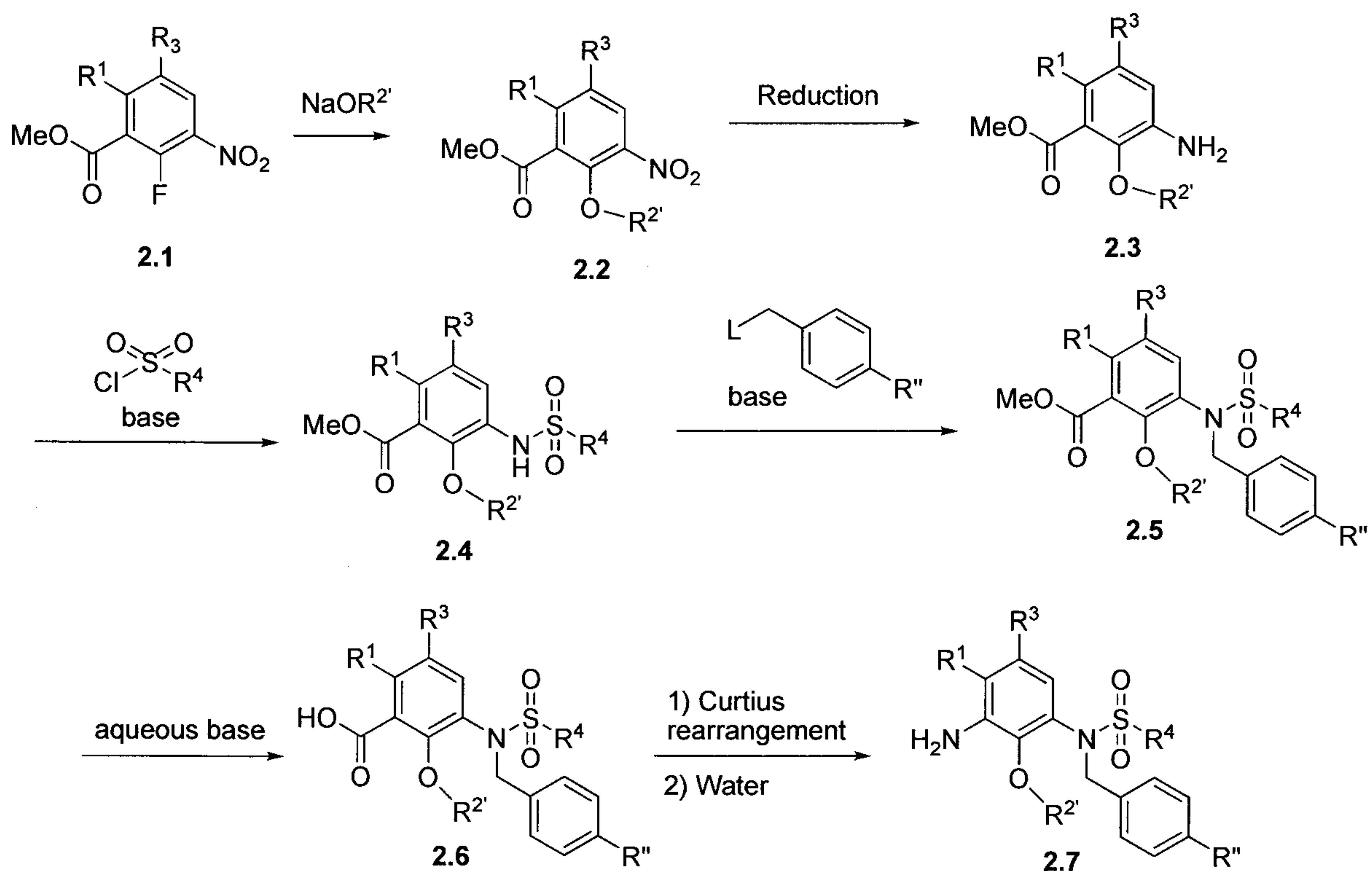
Scheme 2
