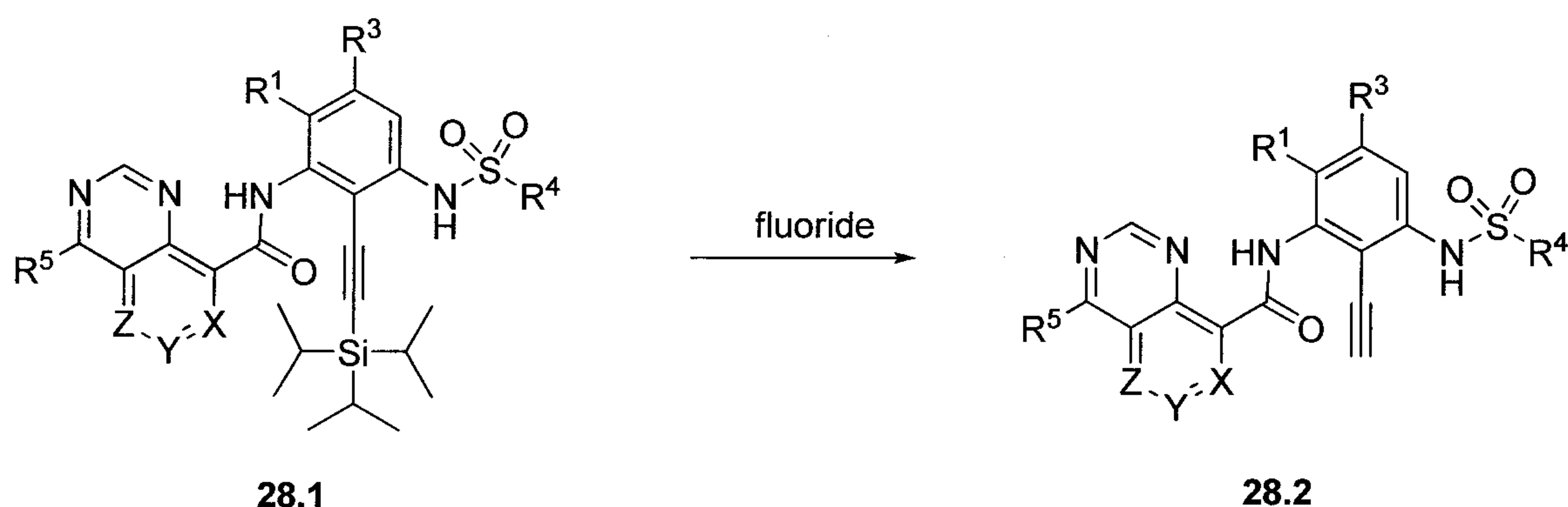
Scheme 28
