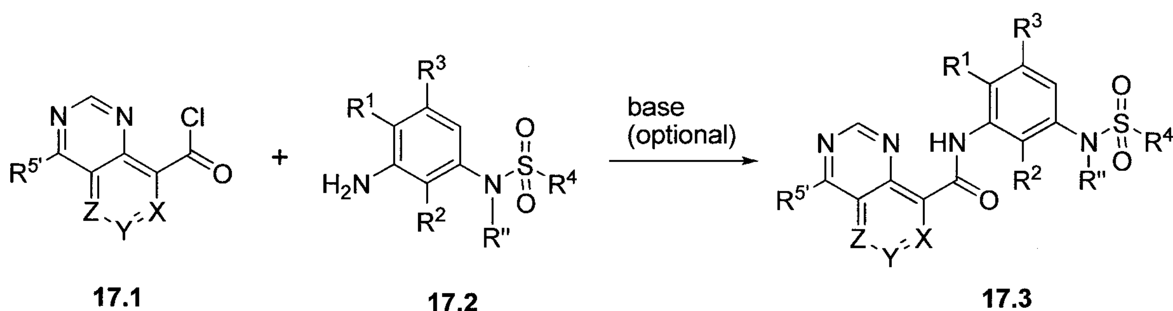
Scheme 17
