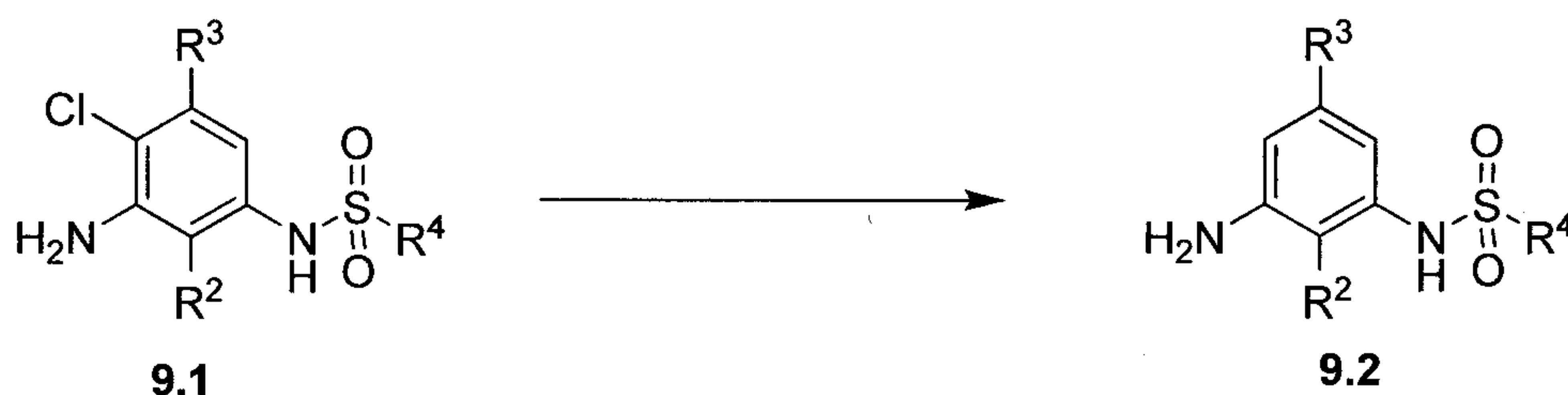
Scheme 9
