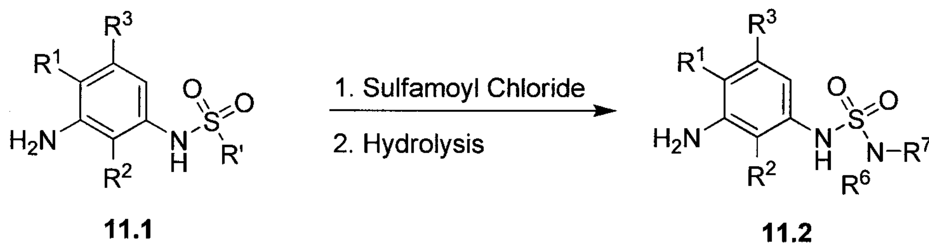
Scheme 11
