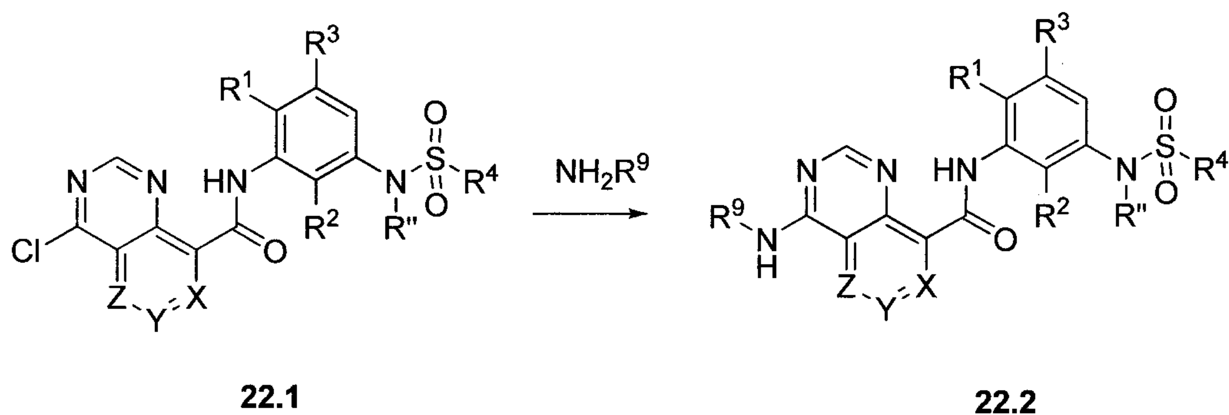
Scheme 22
