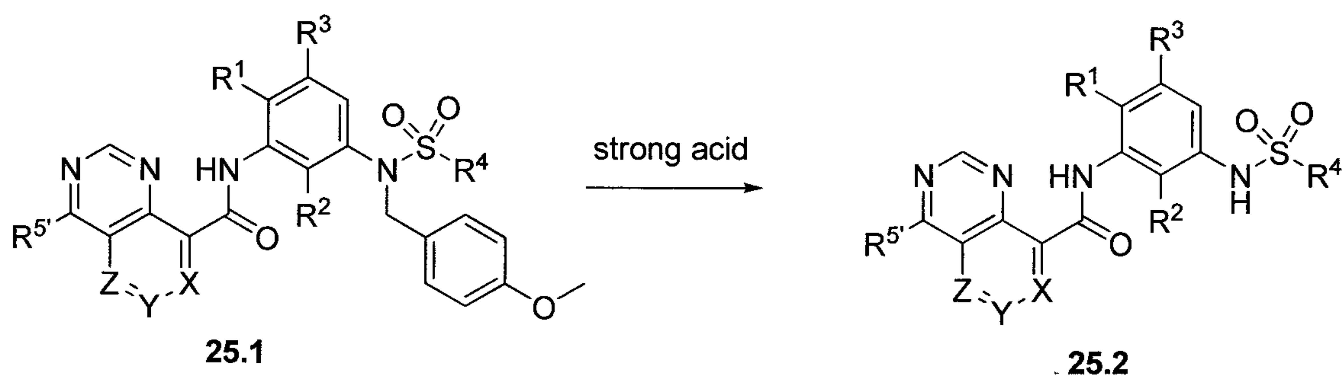
Scheme 25
