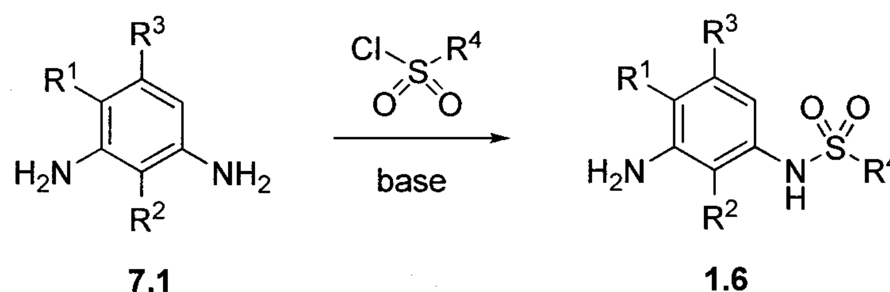
Scheme 7
