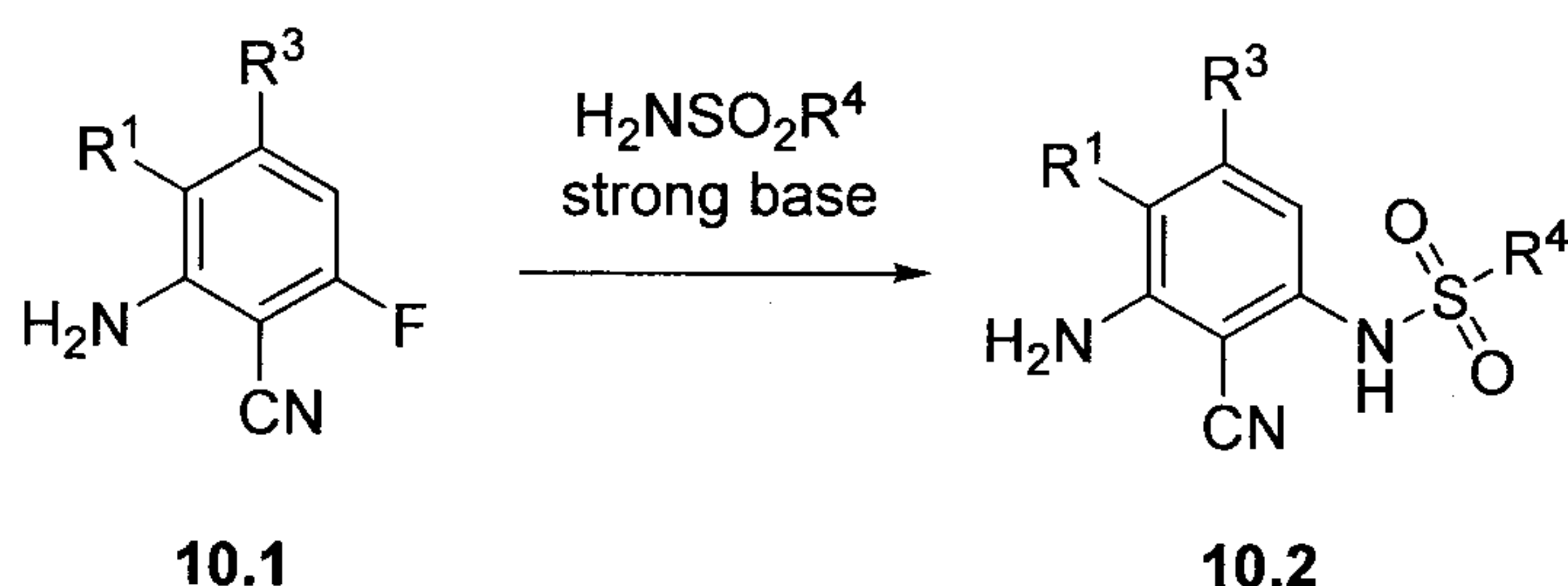
Scheme 10
