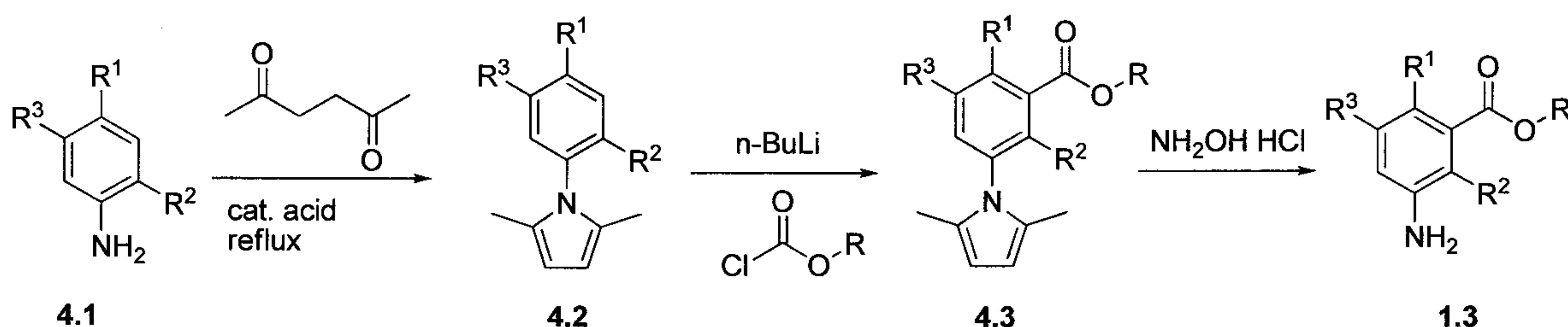
Scheme 4
