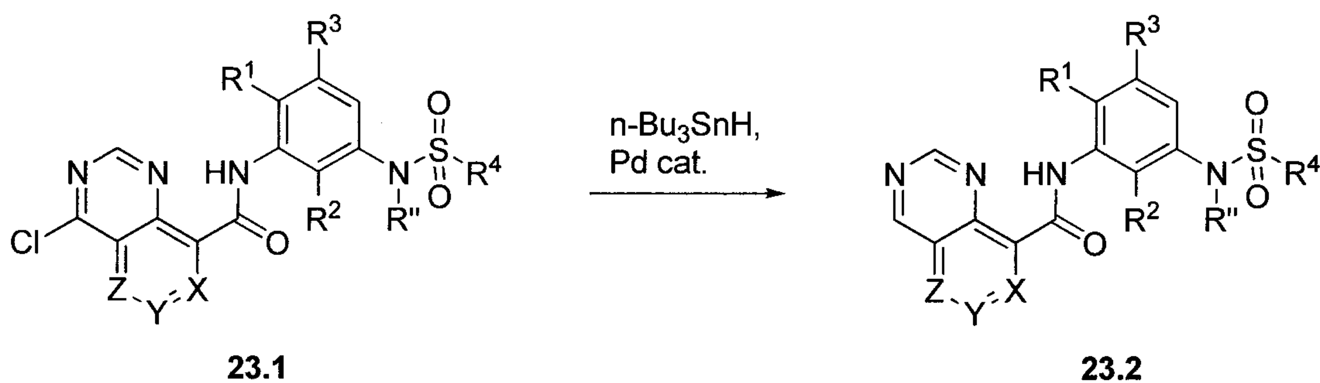
Scheme 23
