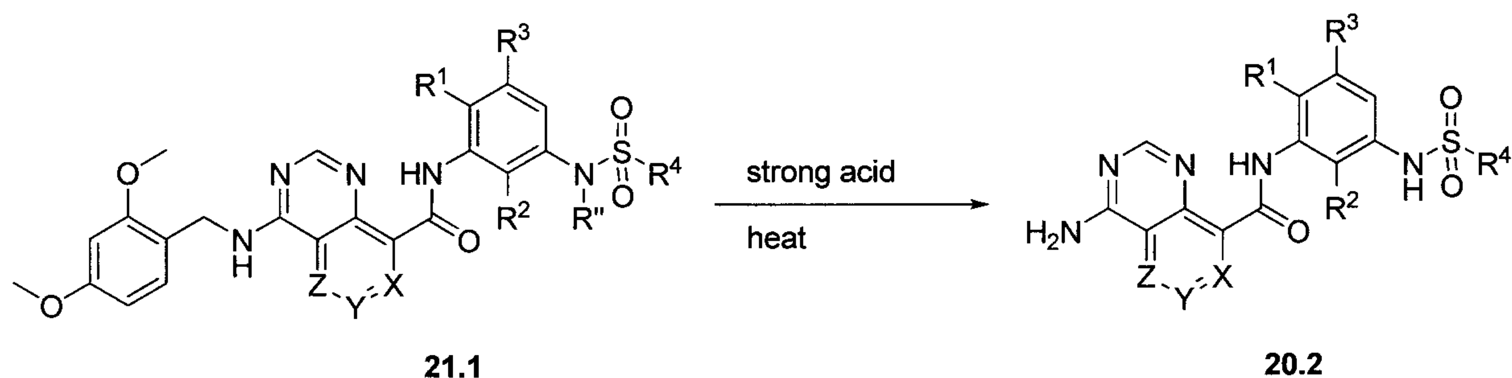
Scheme 21
