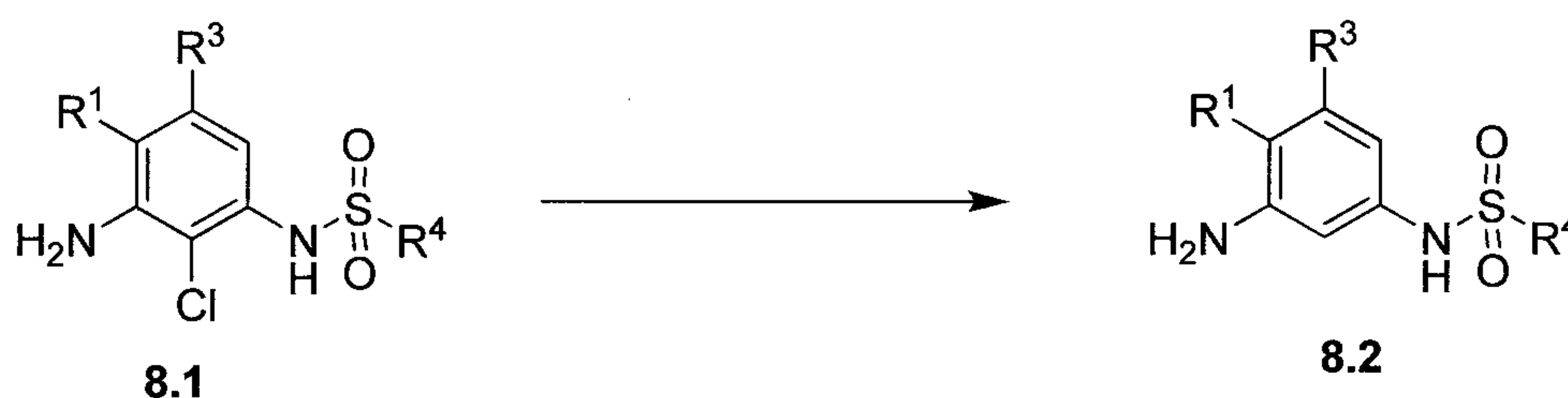
Scheme 8
