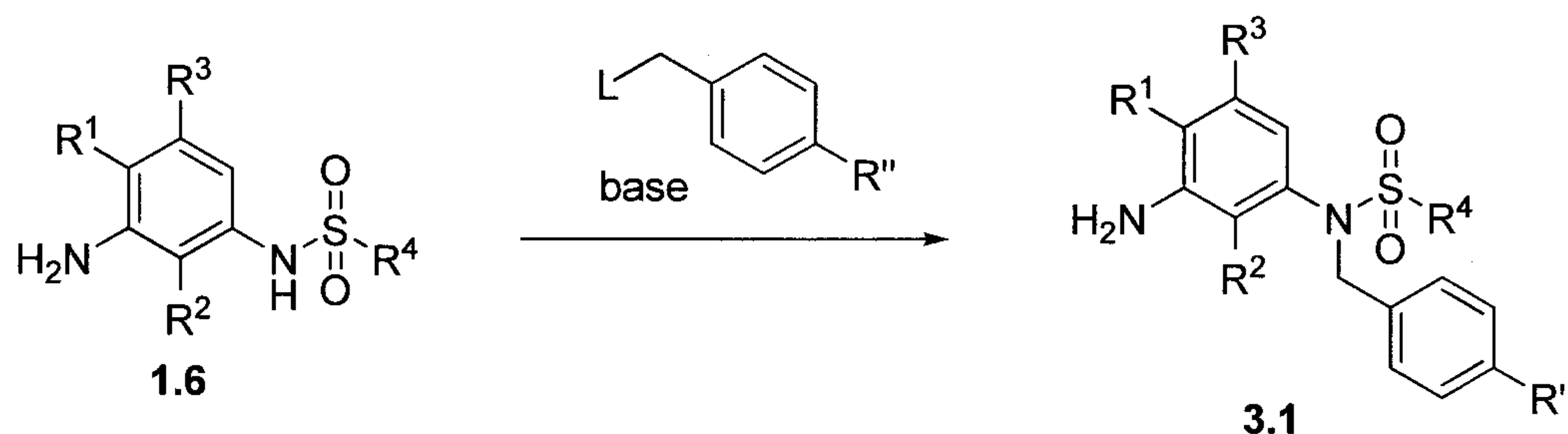
Scheme 3
