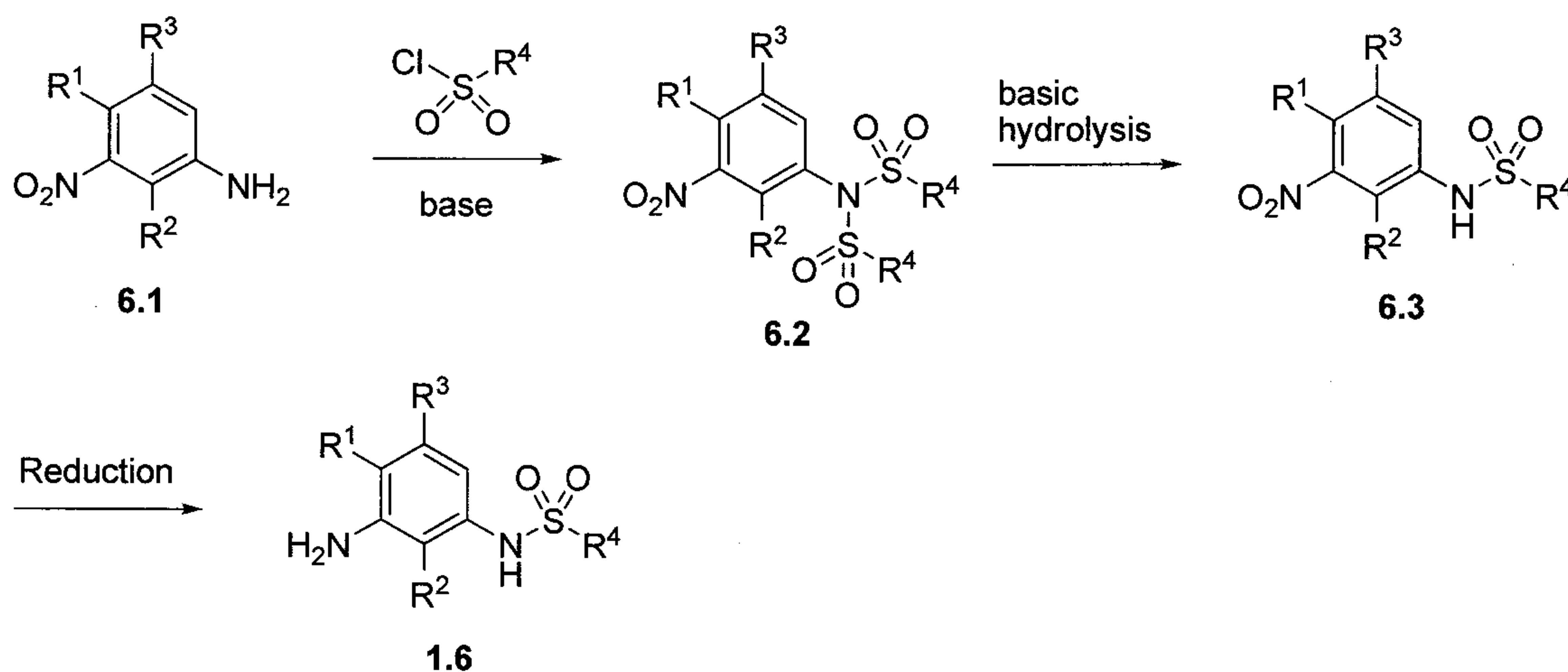
Scheme 6
