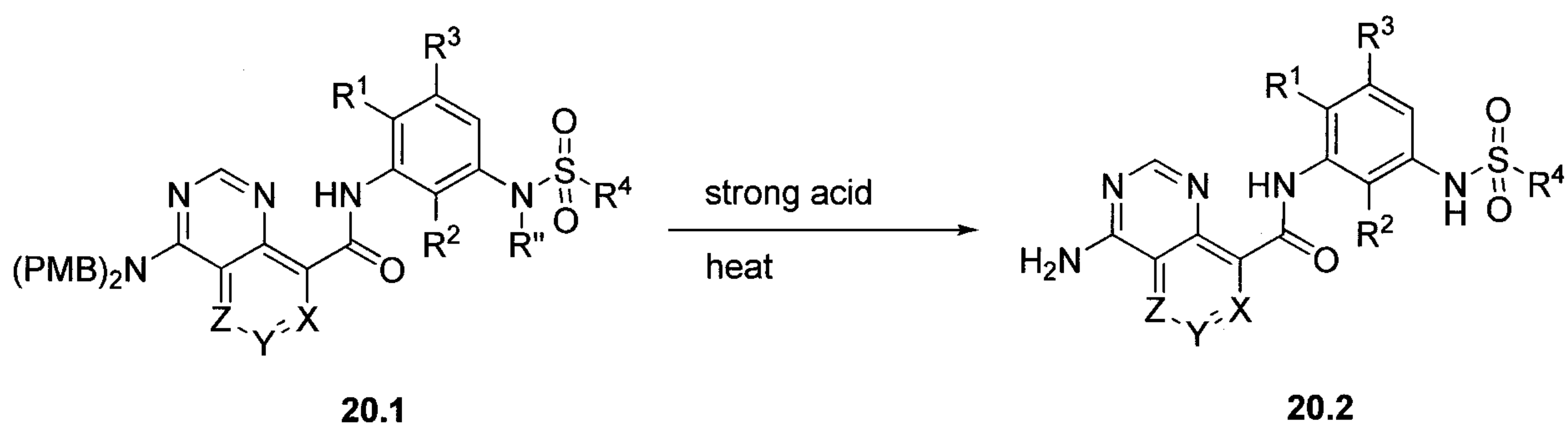
Scheme 20
