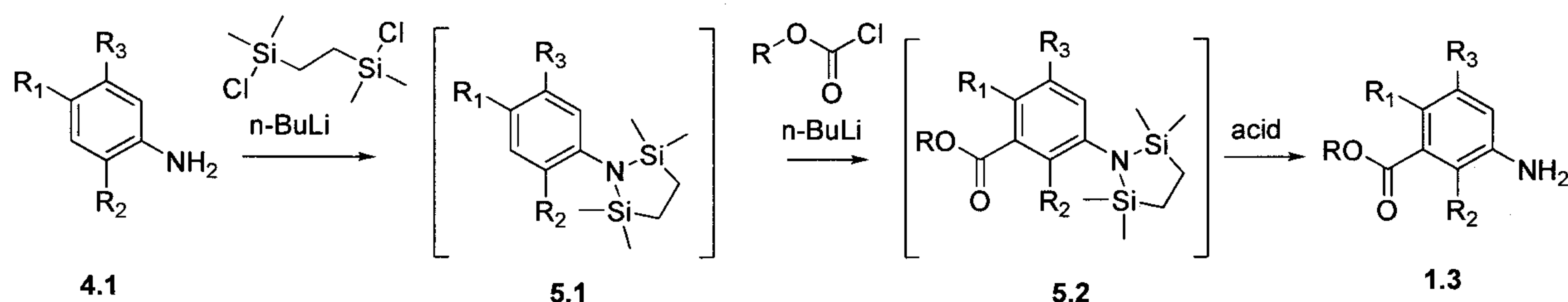
Scheme 5
