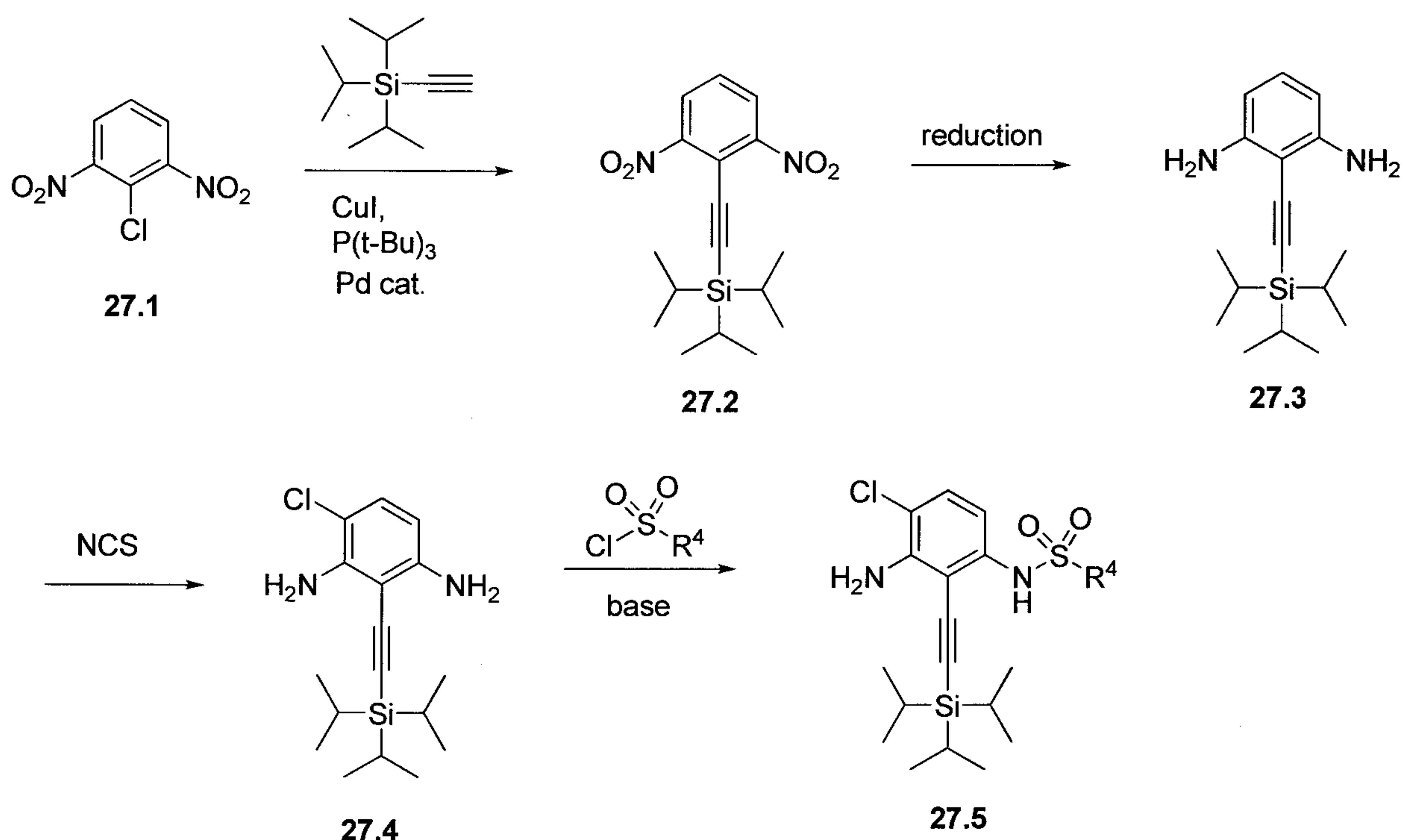
Scheme 27
