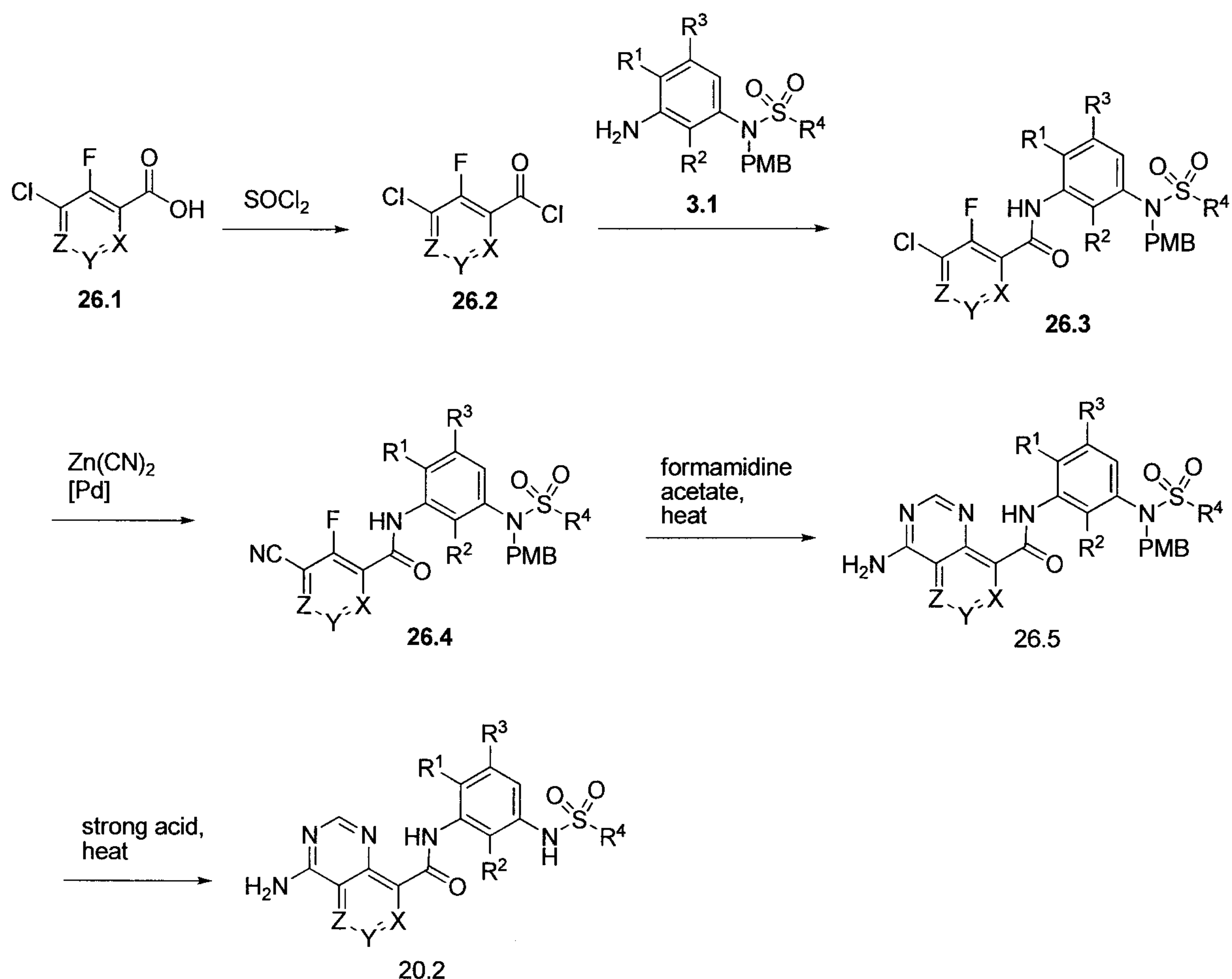
Scheme 26
