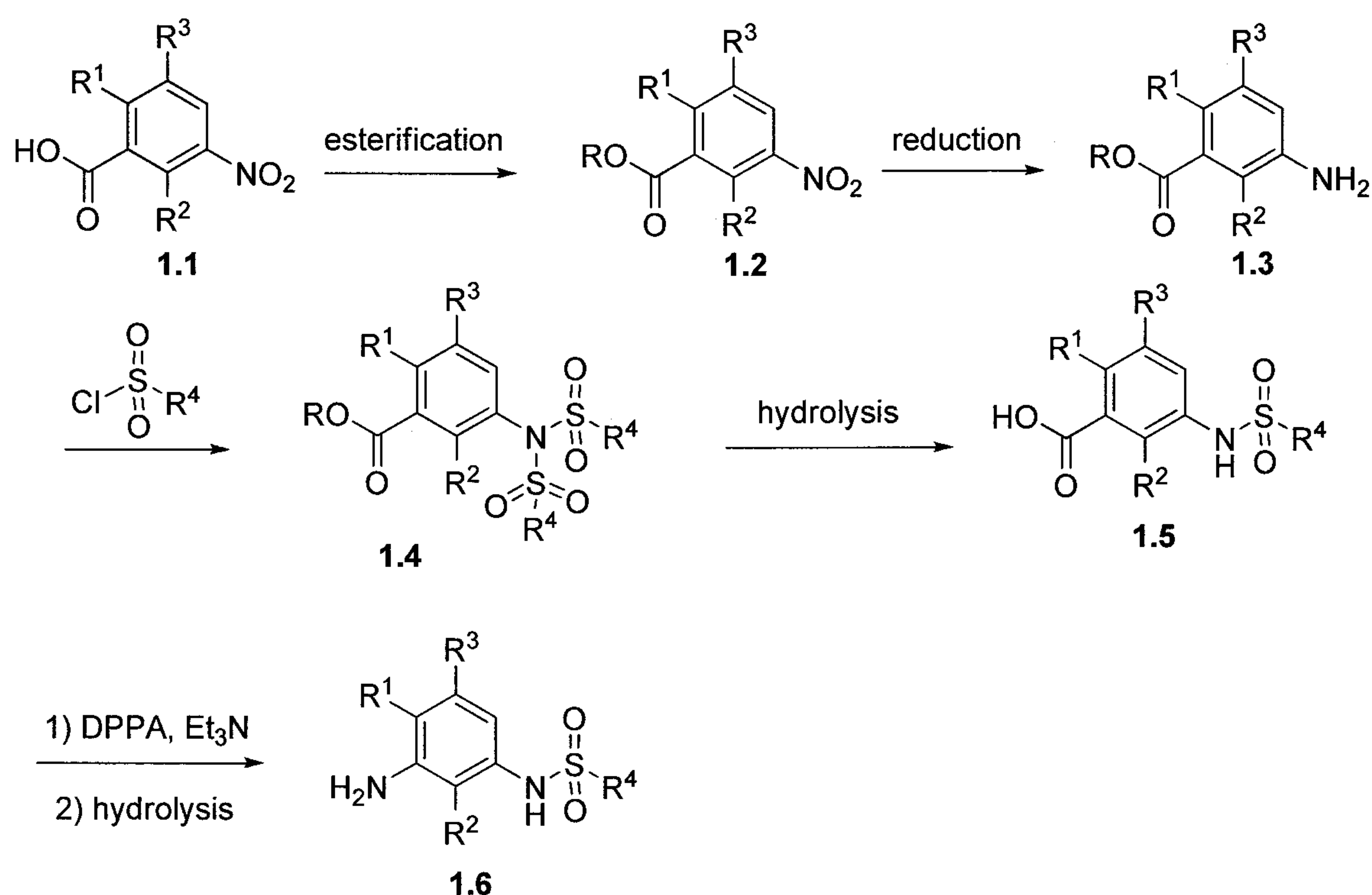
Scheme 1
