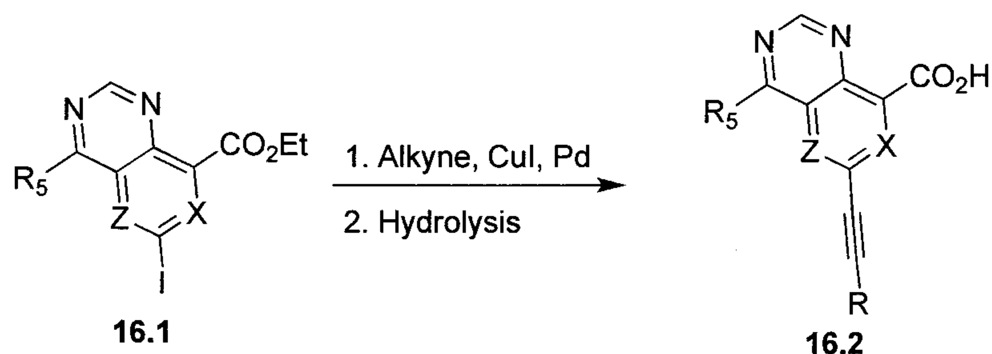
Scheme 16
