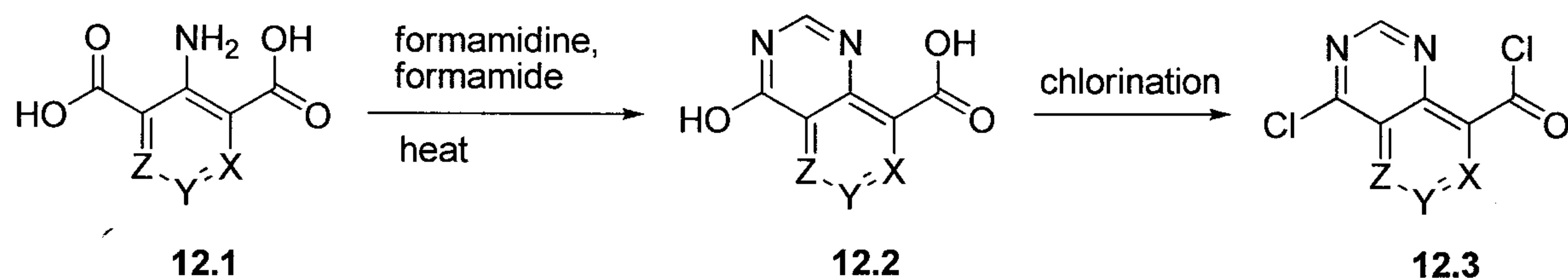
Scheme 12
