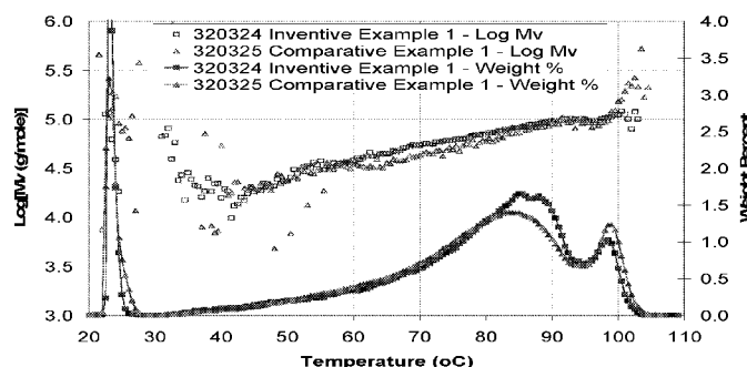
Figure 1: Short Chain Branching Distribution and log Mv data from ATREF For Inventive Resin 1 and Comparative Example 1.
