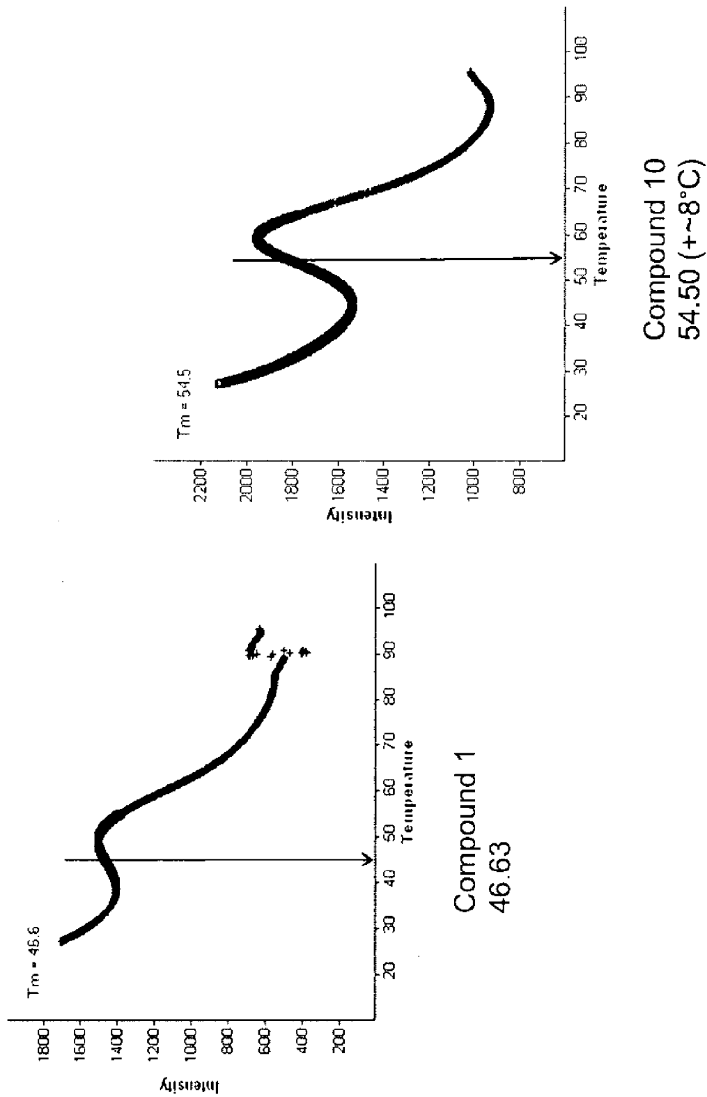
FIG. 4. Thermal Stability by Thermal Scanning Fluorescence (TSF)
