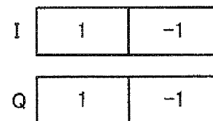
FIG.25B WHEN DATA REPRESENTING "1" IS SENT
