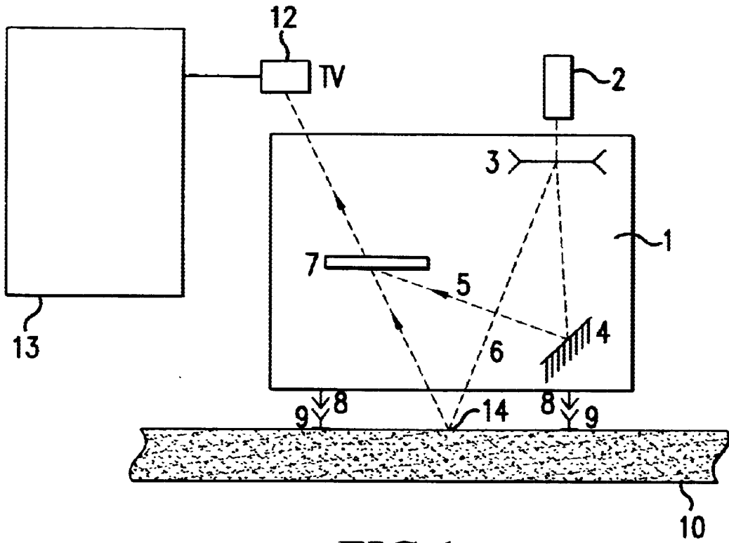
FIG. 1 BACKGROUND ART
