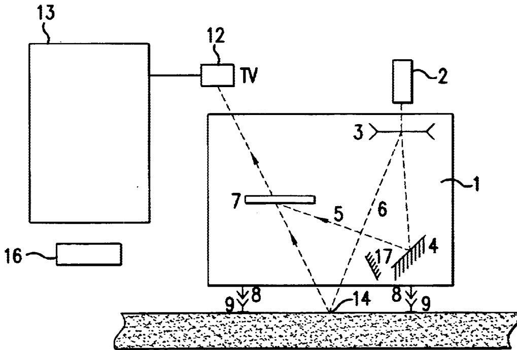
FIG. 4 BACKGROUND ART
