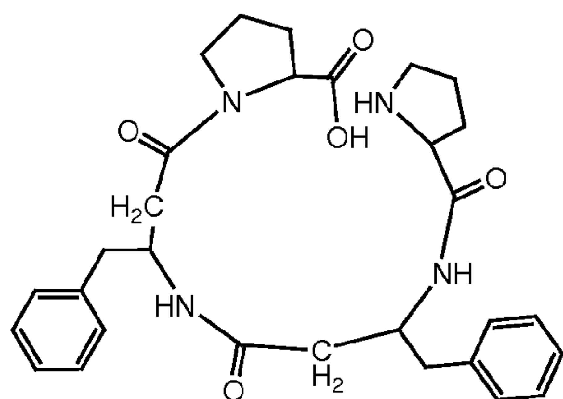
II-4-c ( \text{H-Pro-}\beta^3\text{hoPhe-}\beta^3\text{hoPhe-Pro-OH} ),
