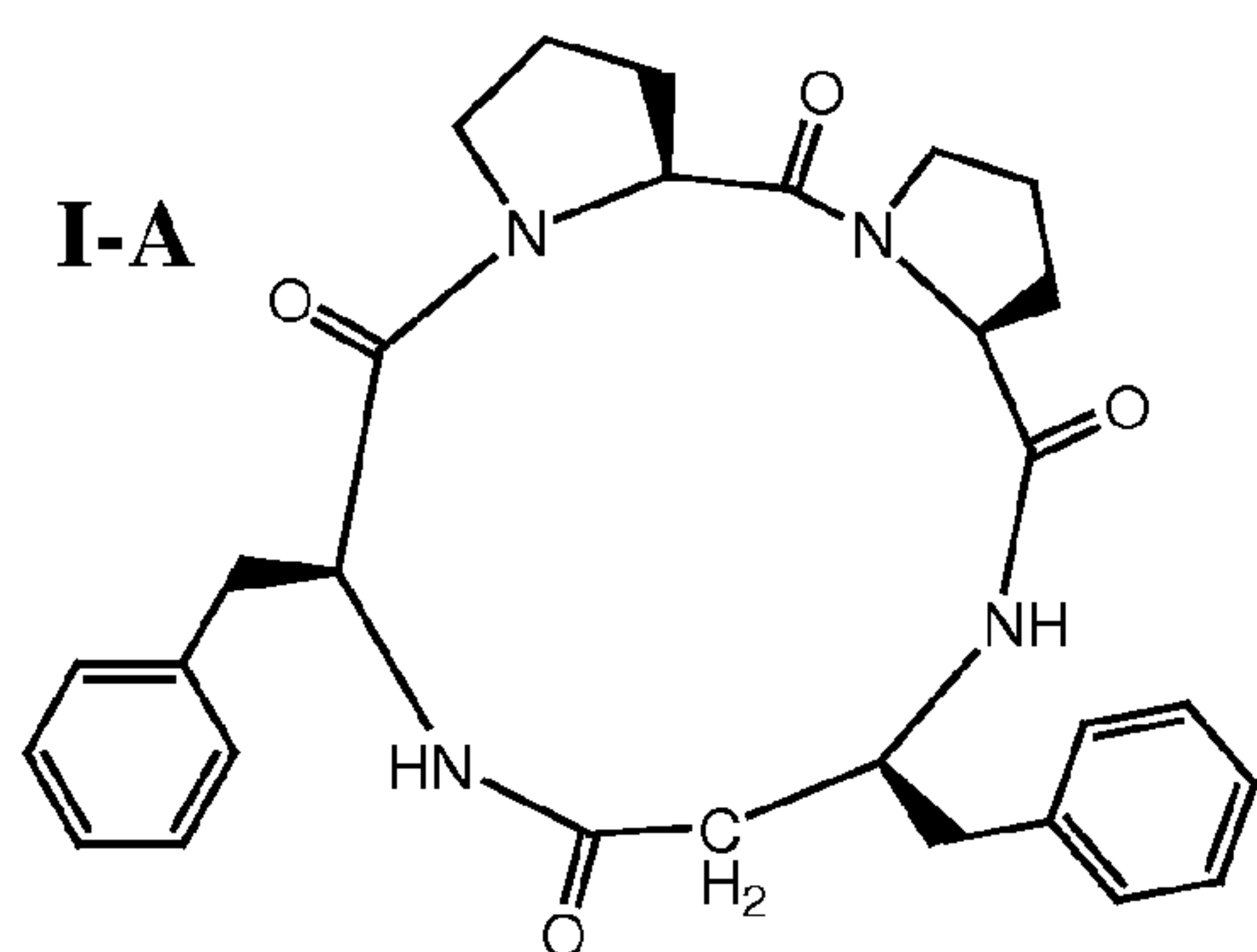
I-A ((cyclic(-(L)-Pro-(L)-Pro-(L)- \beta^3 hoPhe-(L)-Phe-)),
