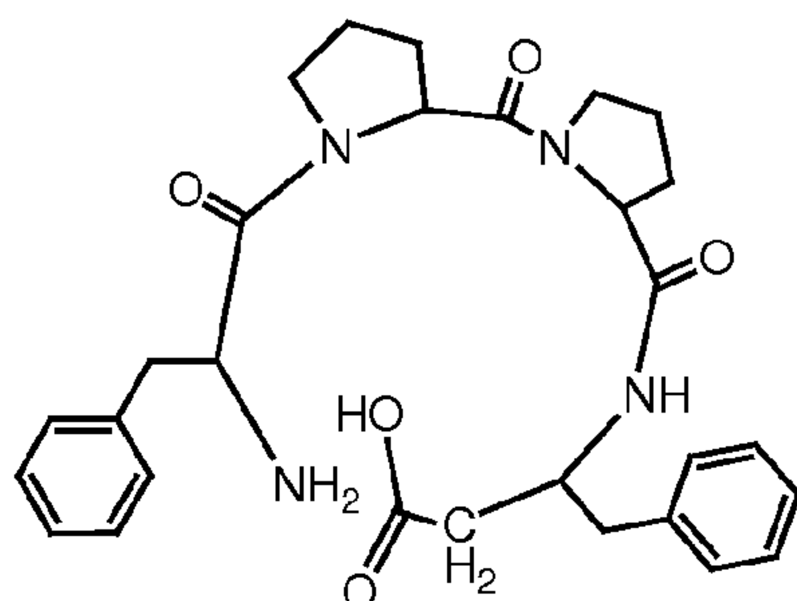
II-2-a (H 2 N-Phe-Pro-Pro-β 3 hoPhe-OH),
