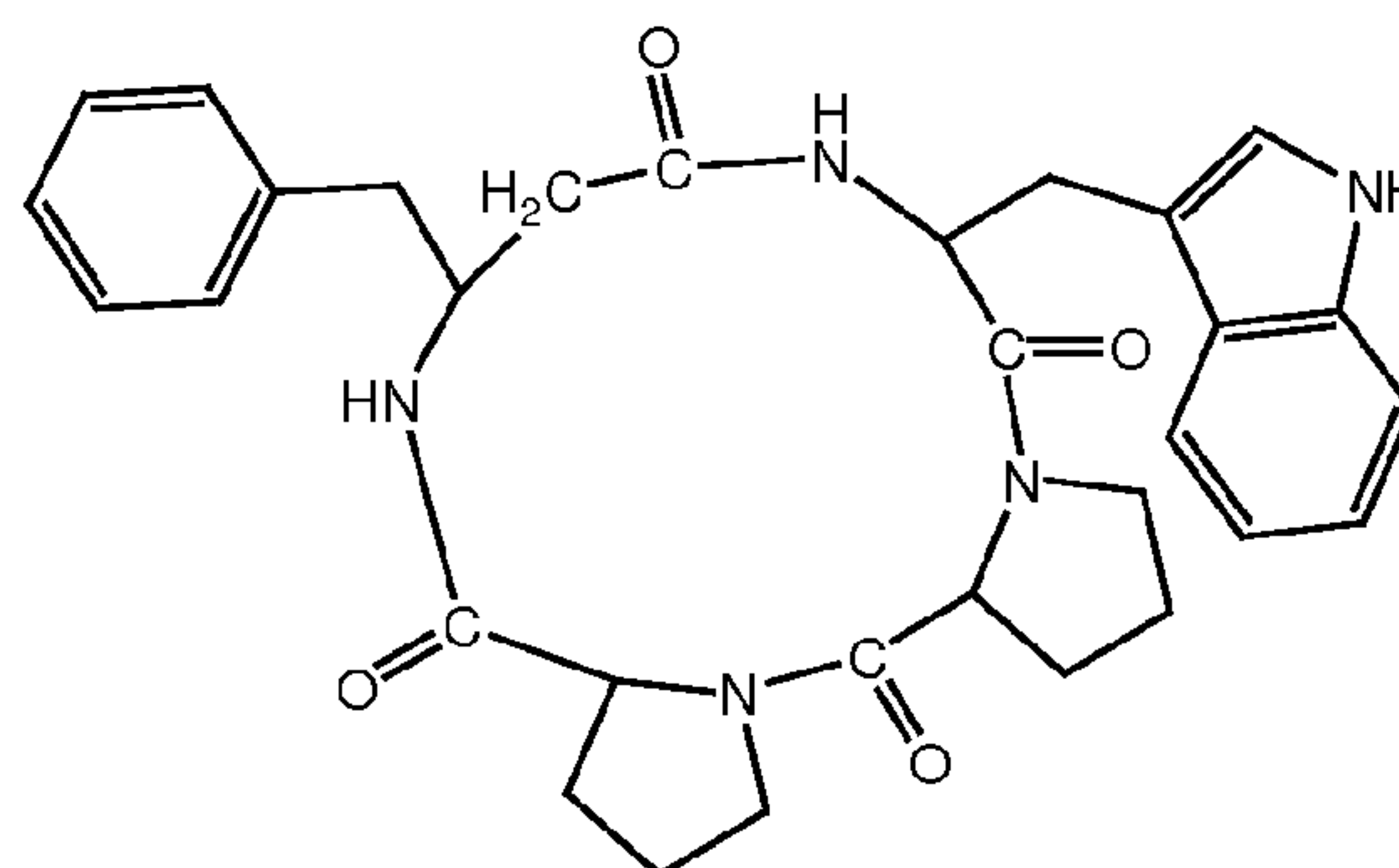
I-4 (cyclic(-Pro-Pro- \beta^3 hoPhe-Trp-)),
