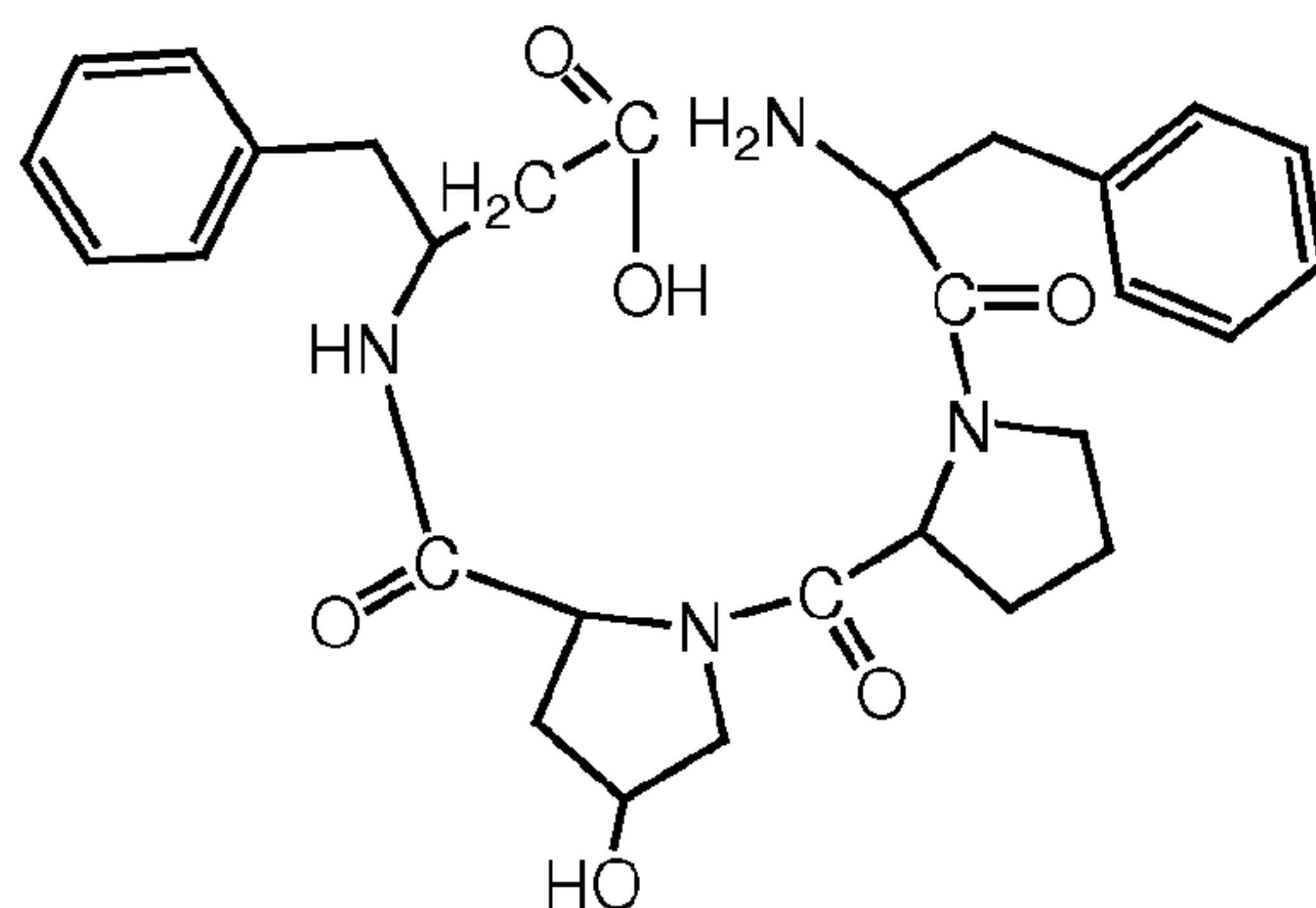
II-2-h (H 2 N-Phe-Pro-Hyp- \beta^3 hoPhe-OH), and
