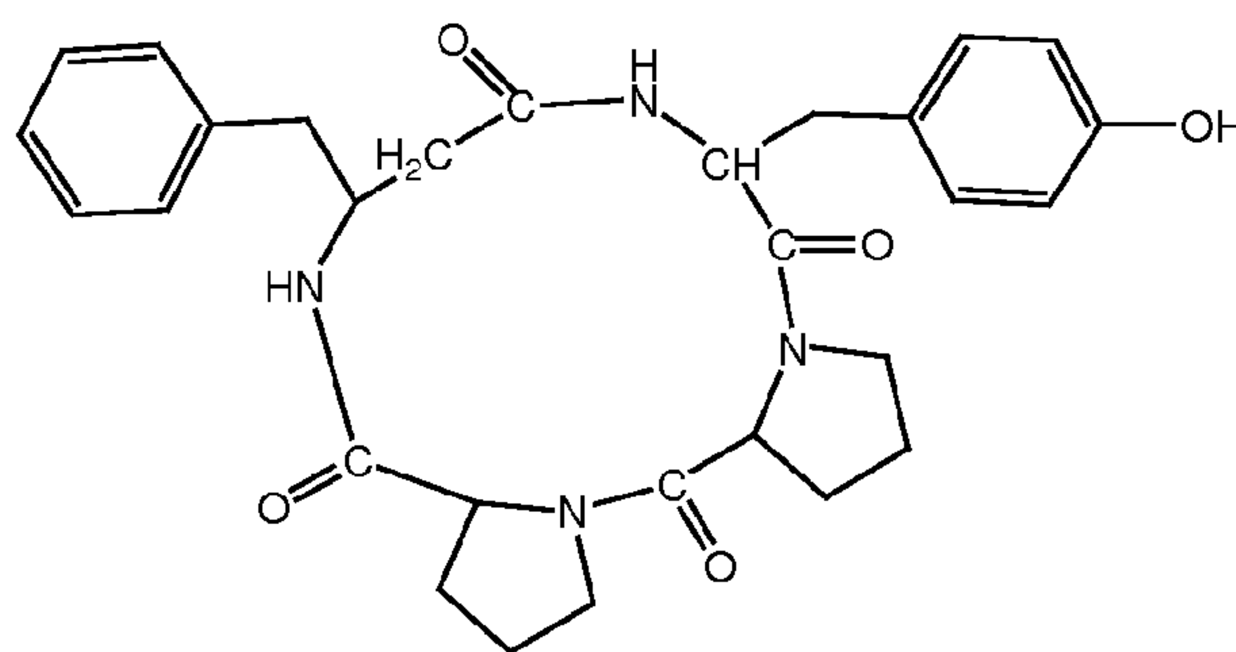
I-5 (cyclic(-Pro-Pro- \beta^3 hoPhe-Tyr-)),
