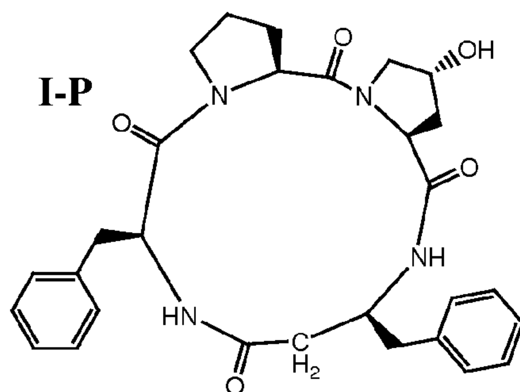
(cyclic[-(L)-Pro-(L)-Pro-(L)- \beta^3 HoPhe-(L)-Tyr(tBu)-]),
