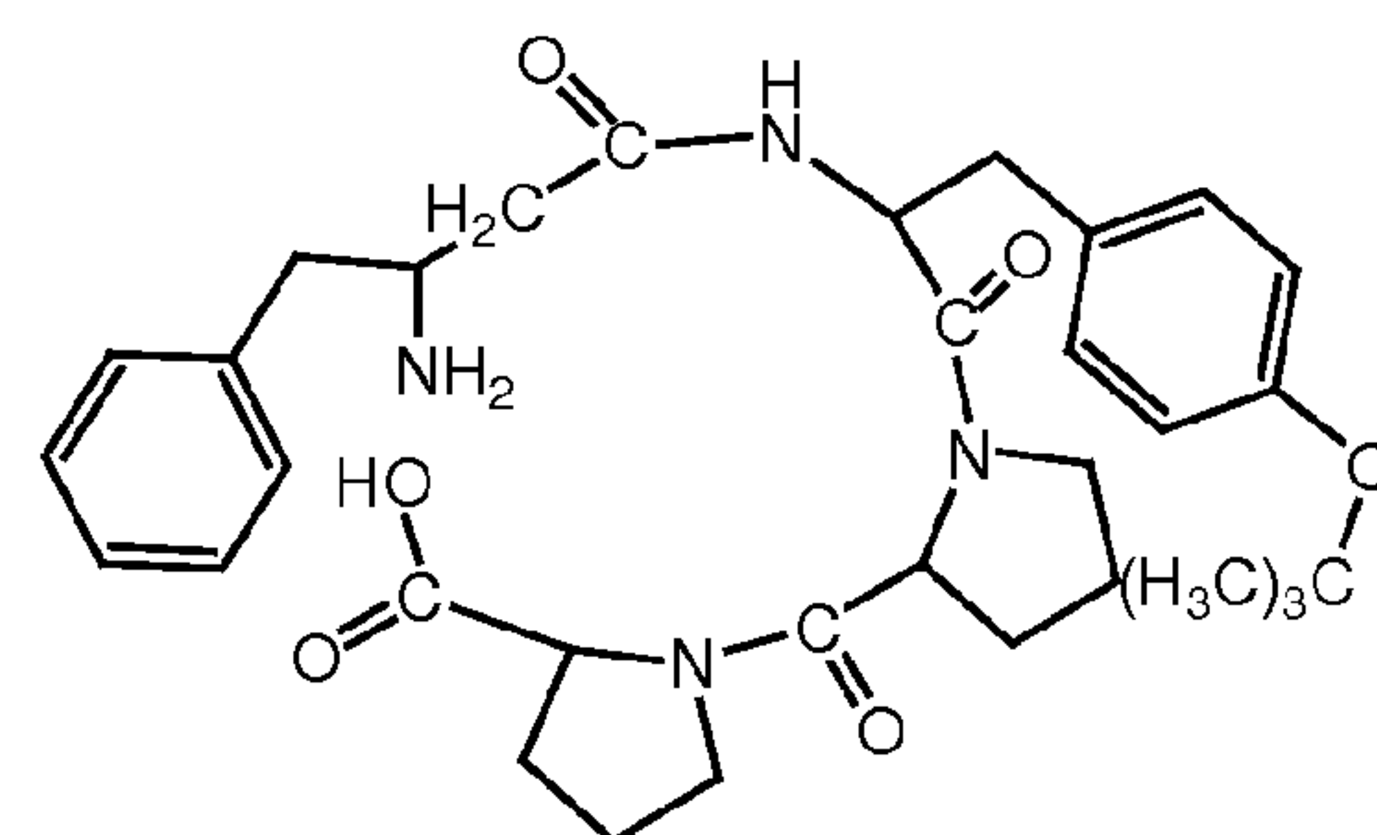
II-3-f (H 2 N- \beta^3 hoPhe-Tyr(t-Bu)-Pro-Pro-OH),
