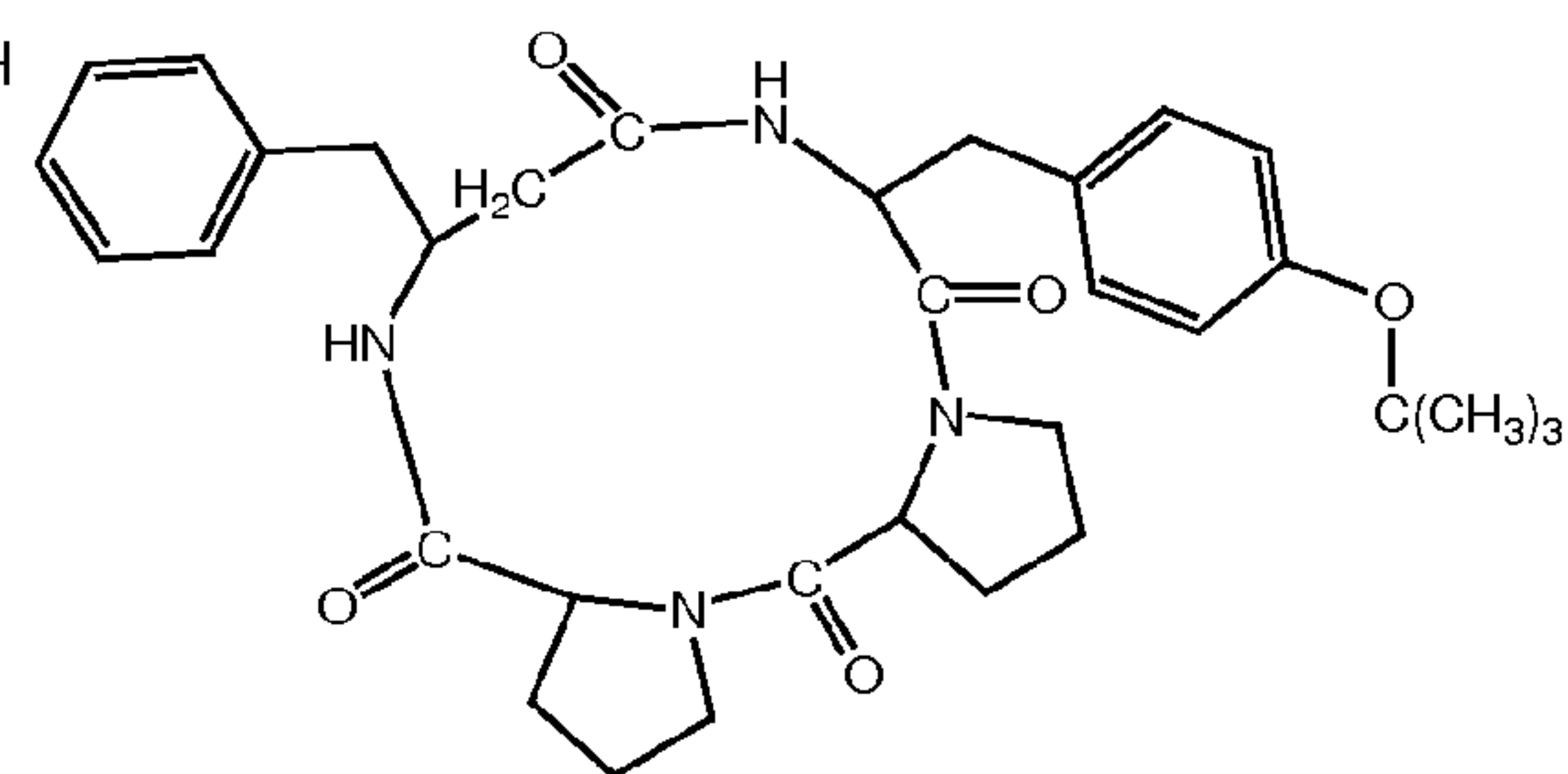
I-6 (cyclic(-Pro-Pro- \beta^3 hoPhe-Tyr(t-Bu)-)),
