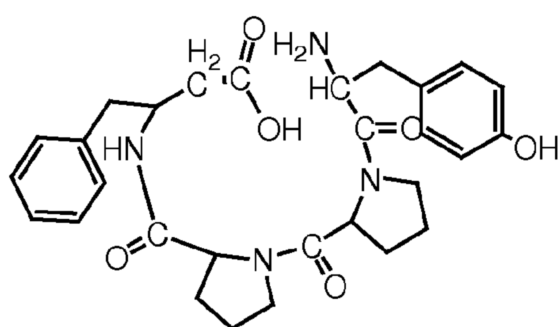
II-2-e (H 2 N-Tyr-Pro-Pro- \beta^3 hoPhe-OH),
