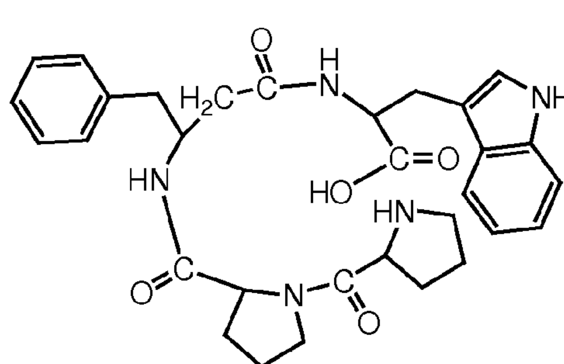
II-1-d ( \text{H-Pro-Pro-}\beta^3\text{hoPhe-Trp-OH} ),
