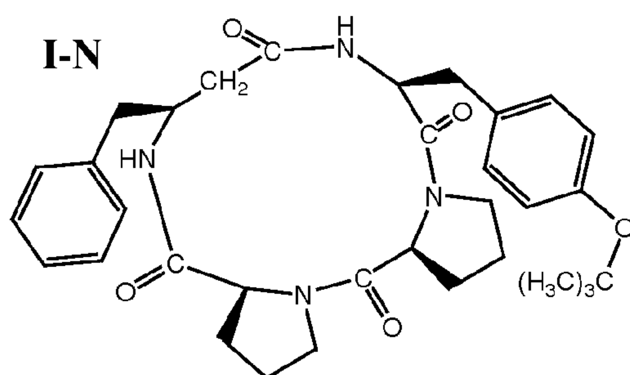
(cyclic[-(L)-Pro-(L)-Pro-(L)- \beta^3 HoPhe-(L)-Tyr(tBu)-]),
