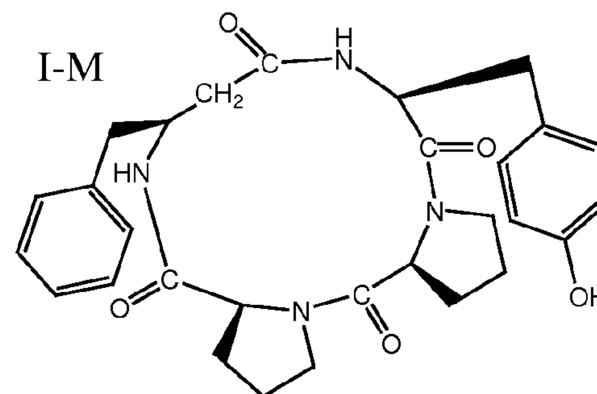
(c(-(L)-Pro-(L)-Pro-(L)- \beta^3 HoPhe-(L)-Tyr-)),
