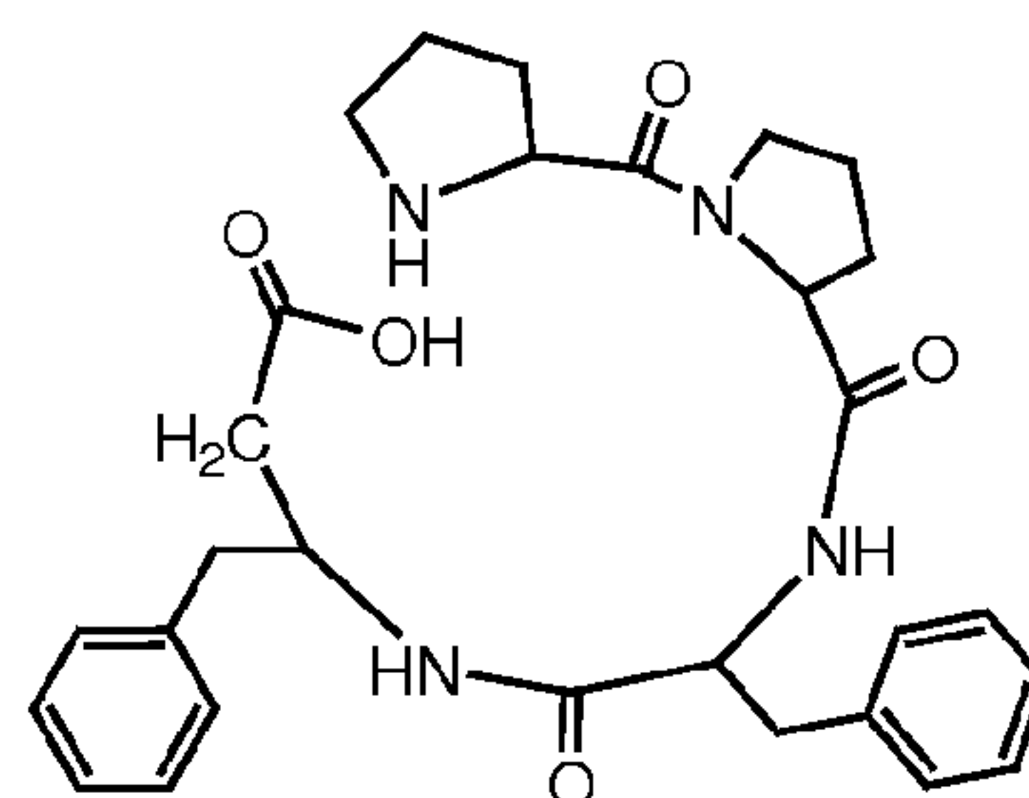
II-1-b (H-Pro-Pro-Phe-β 3 hoPhe-OH),
