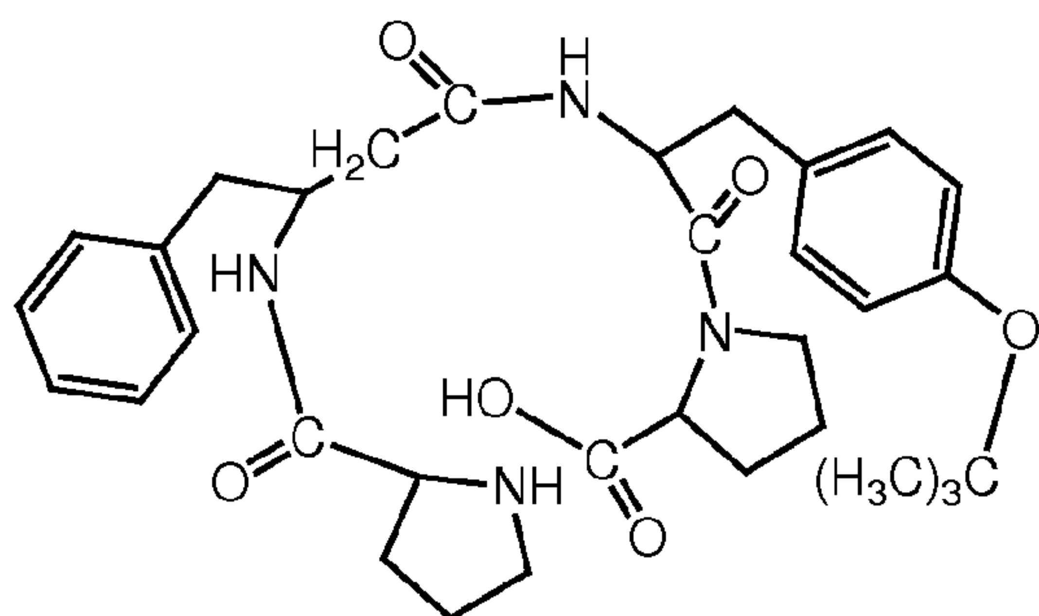
II-4-f (H-Pro- \beta^3 hoPhe-Tyr(t-Bu)-Pro-OH),
