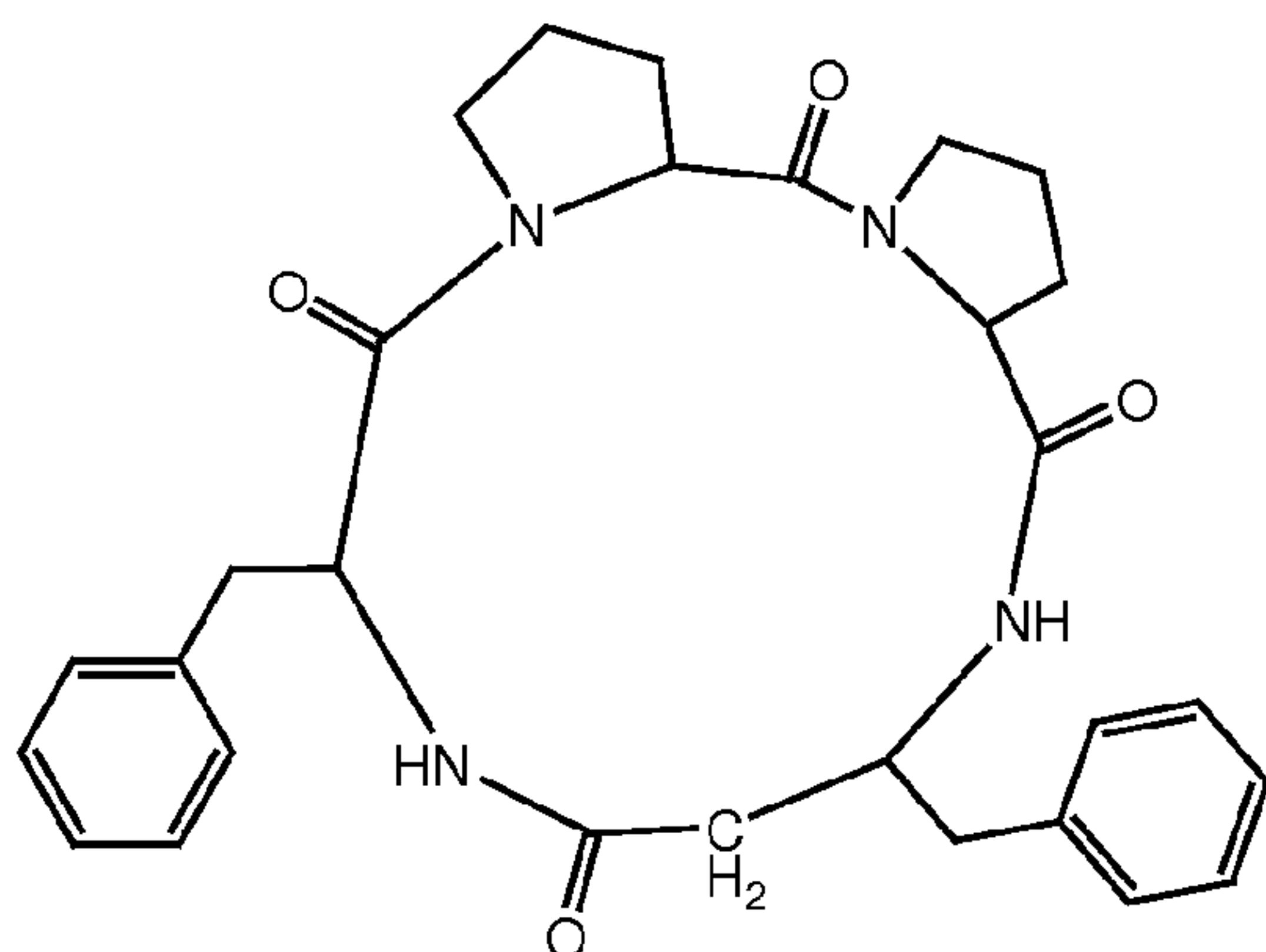
I-1 (cyclic(-Pro-Pro- \beta^3 hoPhe-Phe-)),
