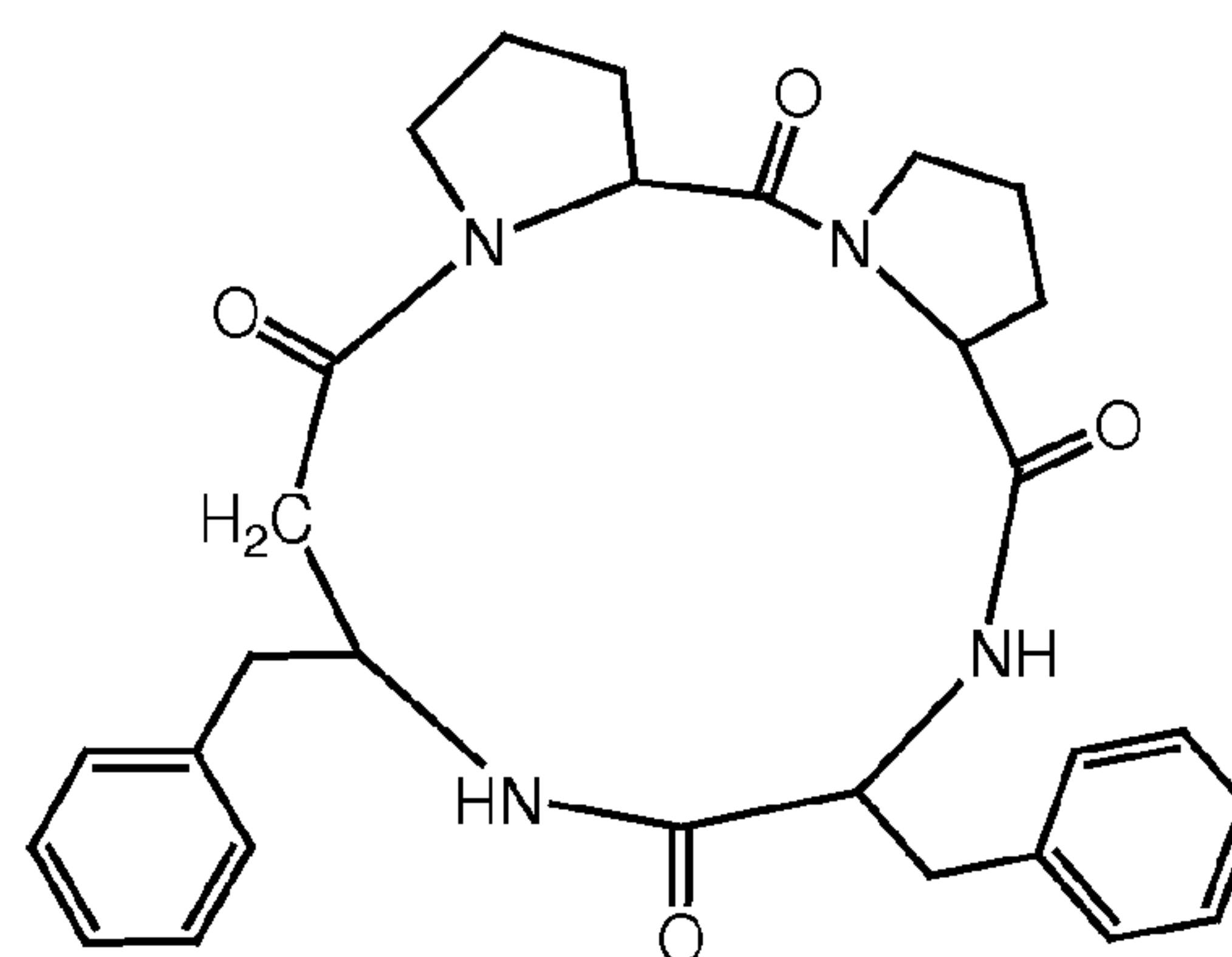
I-2 (cyclic(-Pro-Pro-Phe- \beta^3 hoPhe-)),
