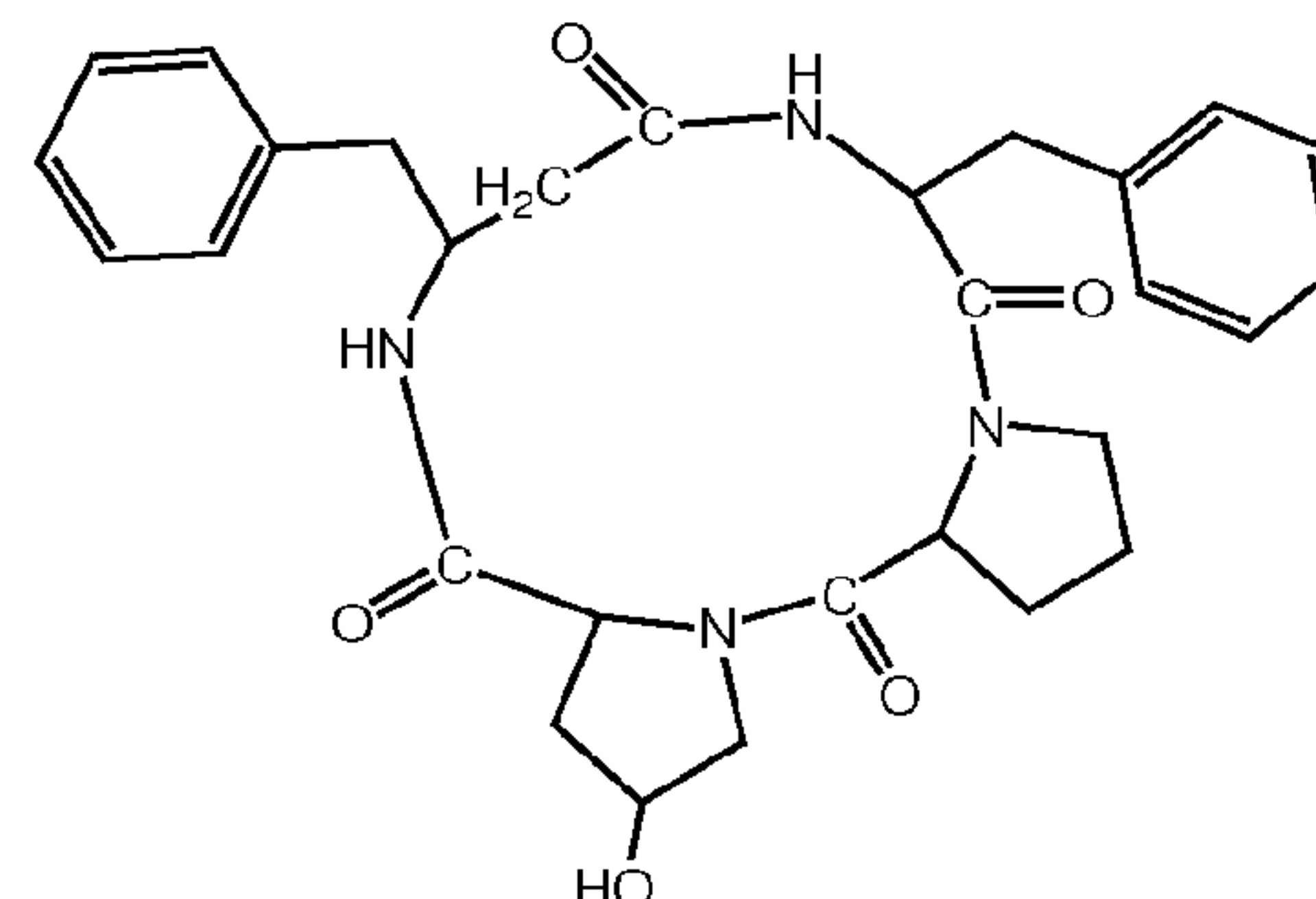
I-7 (cyclic(-Pro-Pip- \beta^3 hoPhe-Phe-)) and
