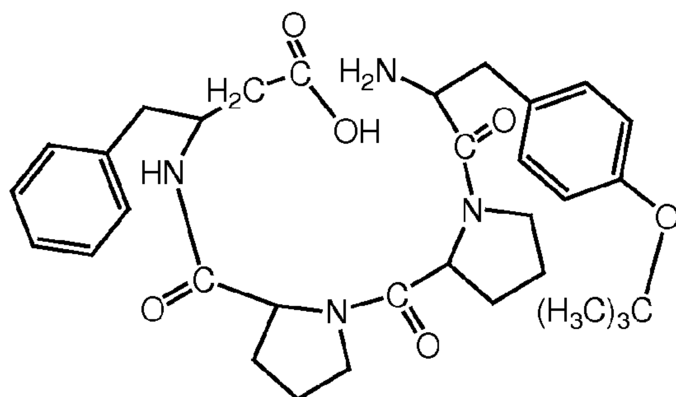
II-2-f (H 2 N-Tyr(t-Bu)-Pro-Pro- \beta^3 hoPhe-OH),
