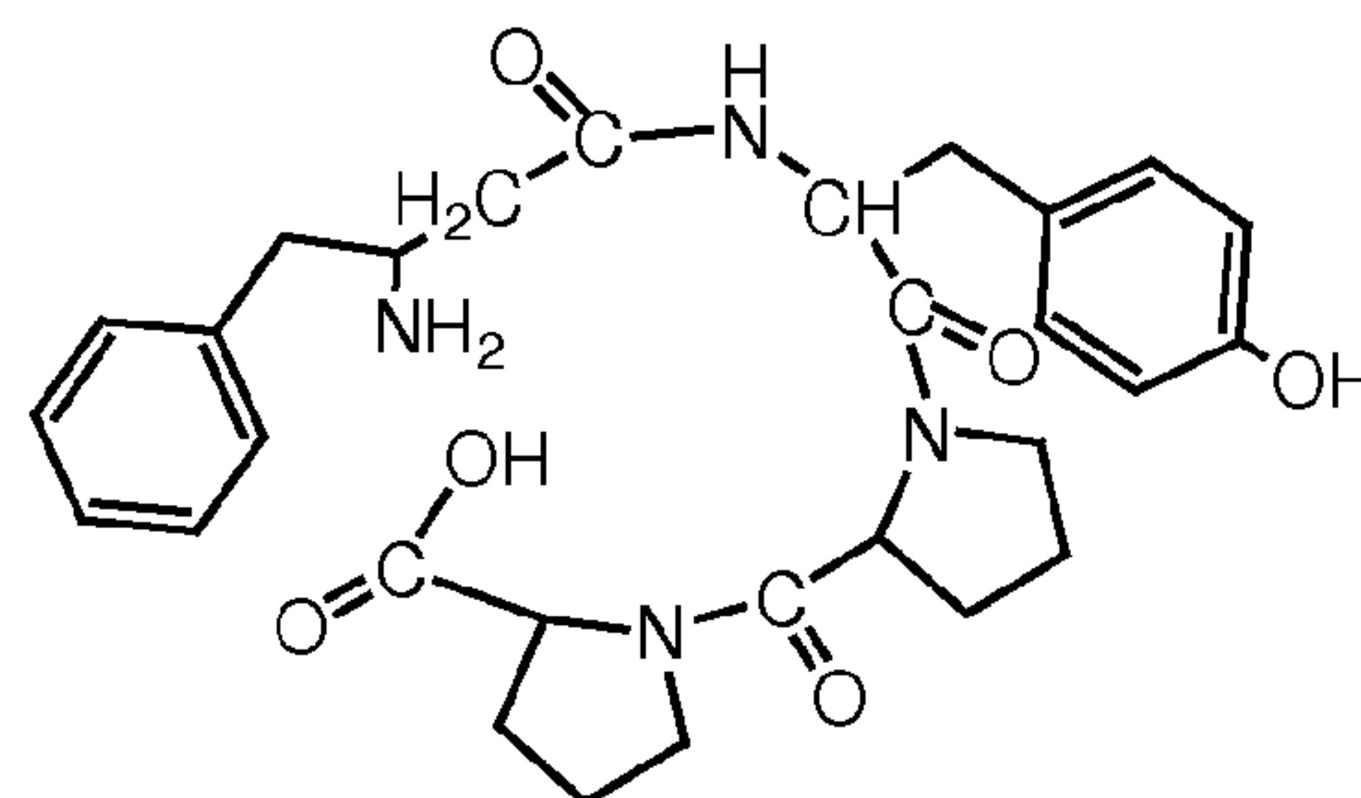
II-3-e (H 2 N- \beta^3 hoPhe-Tyr-Pro-Pro-OH),
