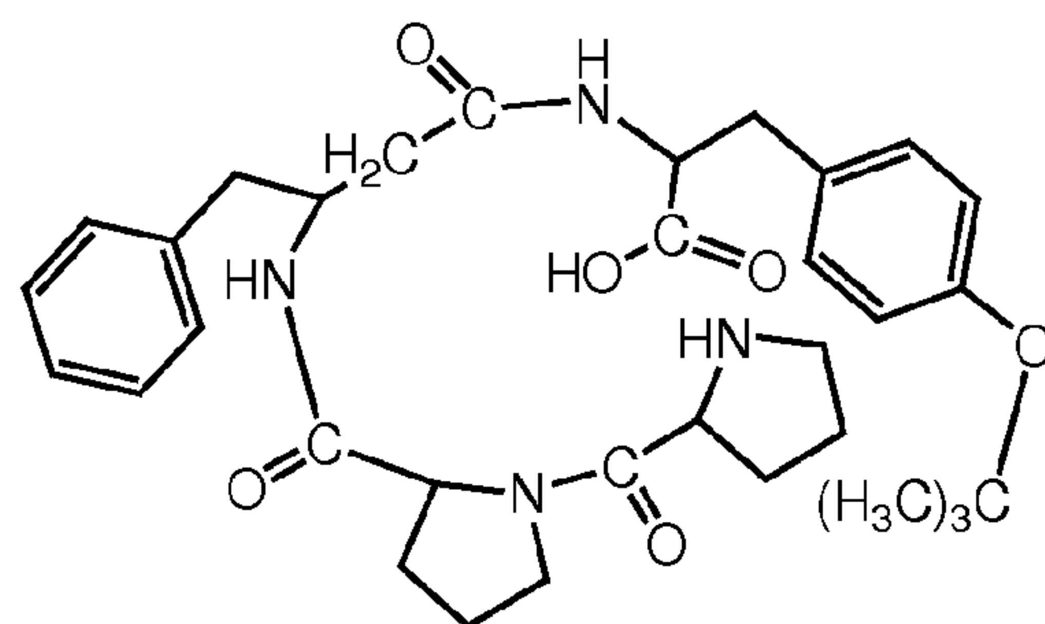
II-1-f (H-Pro-Pro- \beta^3 hoPhe-Tyr(t-Bu)-OH),
