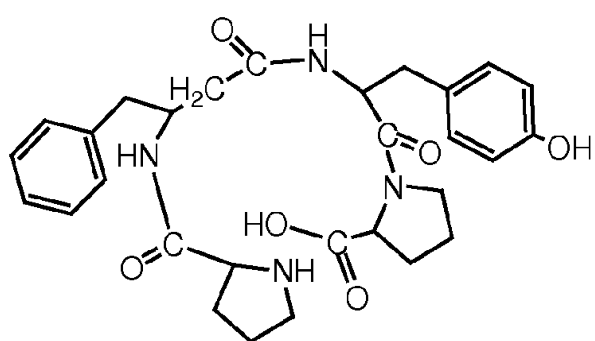
II-4-e (H-Pro- \beta^3 hoPhe-Tyr-Pro-OH),
