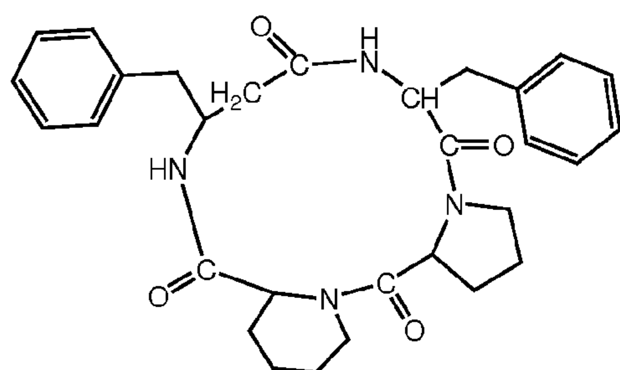
I-7 (cyclic(-Pro-Pip- \beta^3 hoPhe-Phe-)) and
