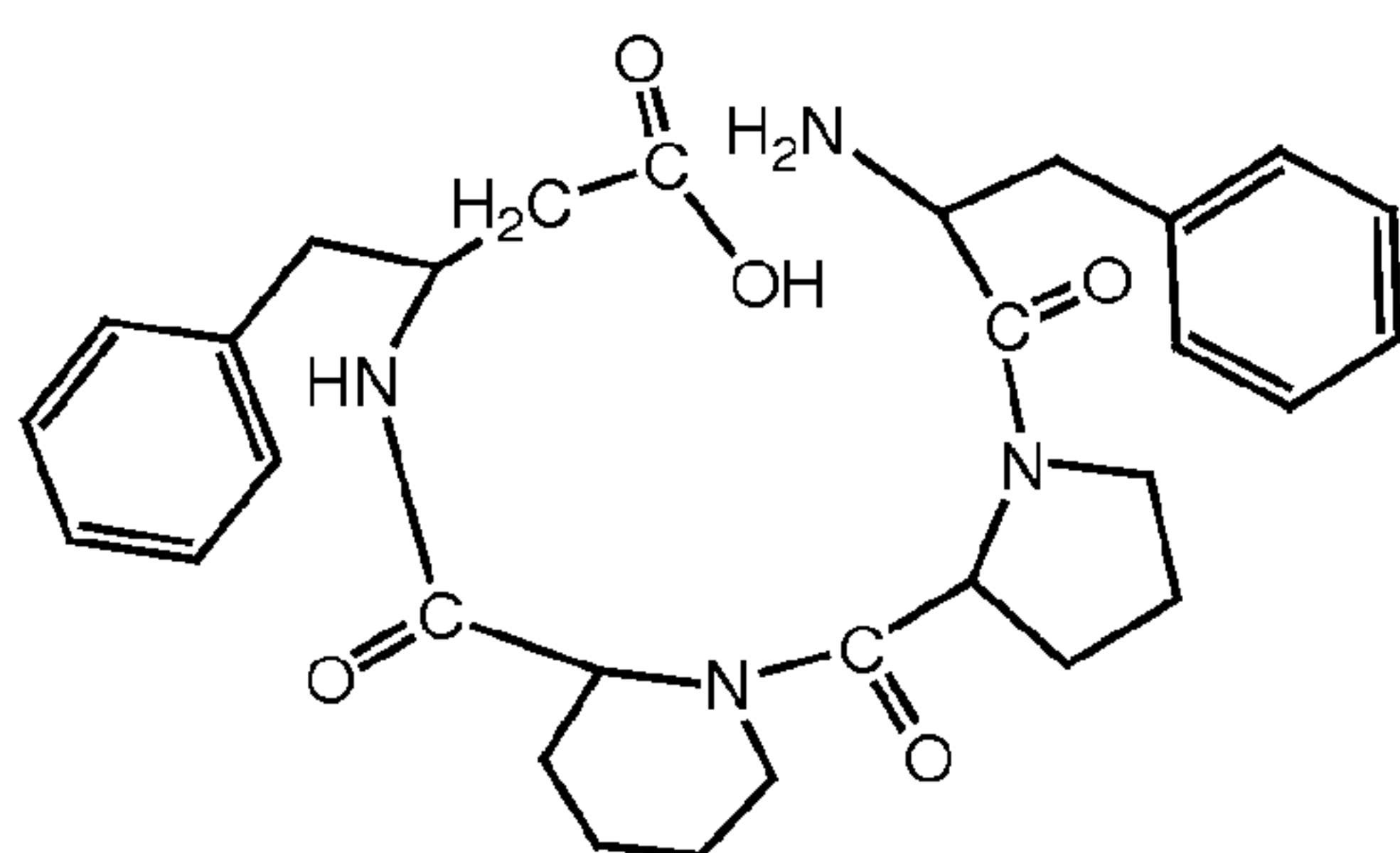
II-2-g (H 2 N-Phe-Pro-Pip- \beta^3 hoPhe-OH),
