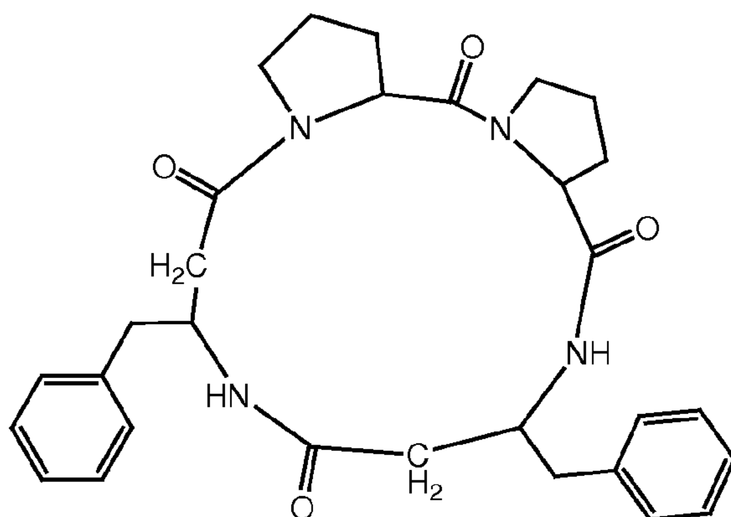
I-3 (cyclic(-Pro-Pro- \beta^3 hoPhe- \beta^3 hoPhe-)),
