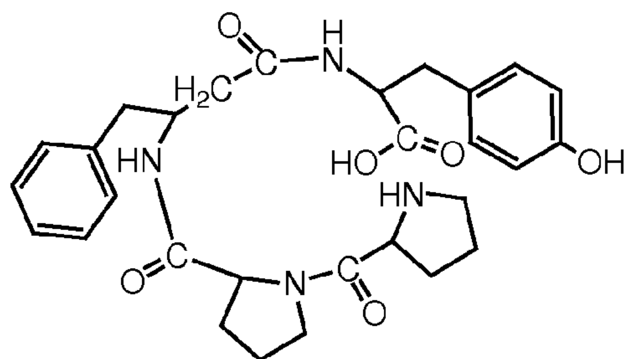
II-1-e (H-Pro-Pro- \beta^3 hoPhe-Tyr-OH),
