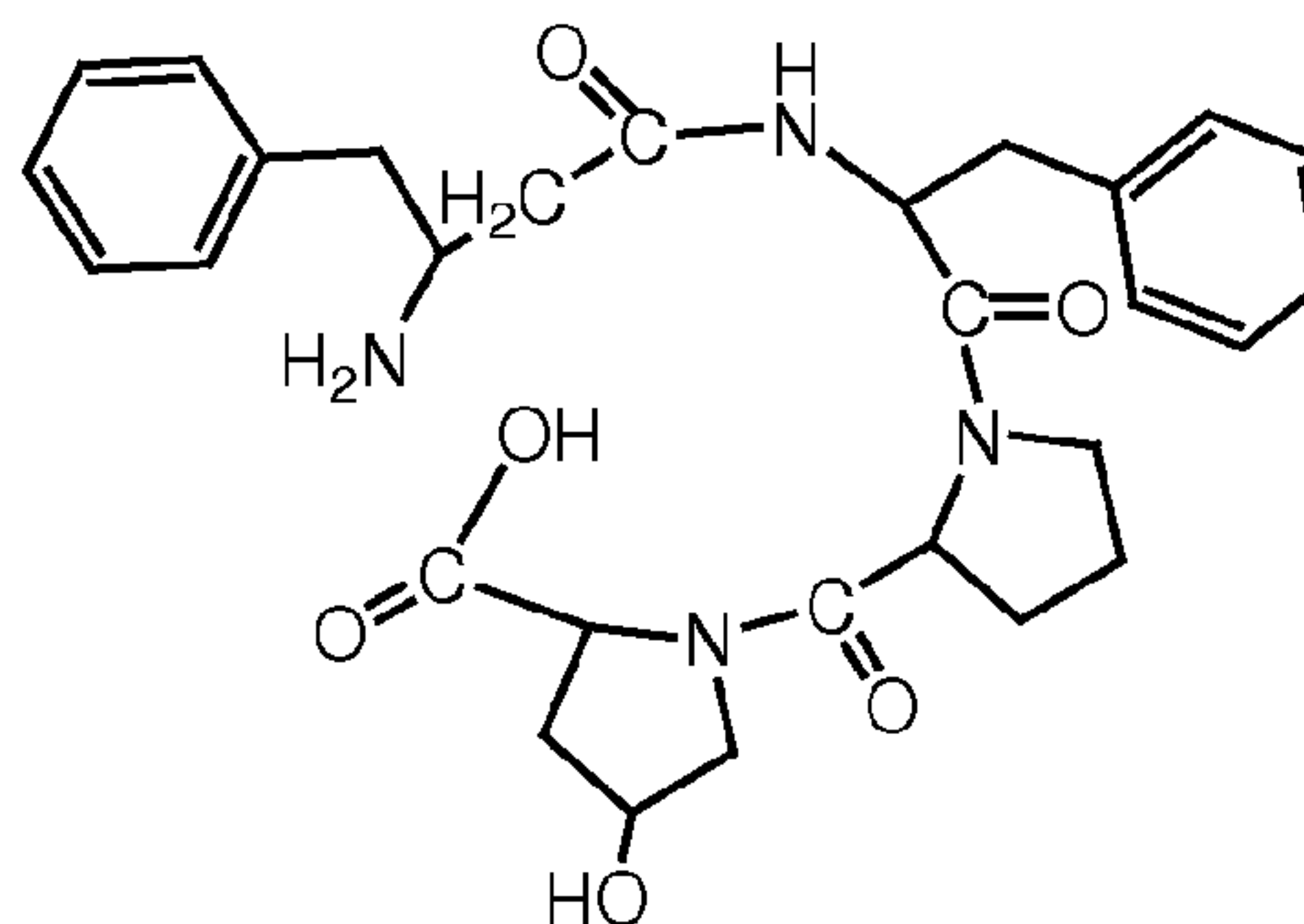
II-3-h (H 2 N- \beta^3 hoPhe-Phe-Pro-Hyp-OH).
