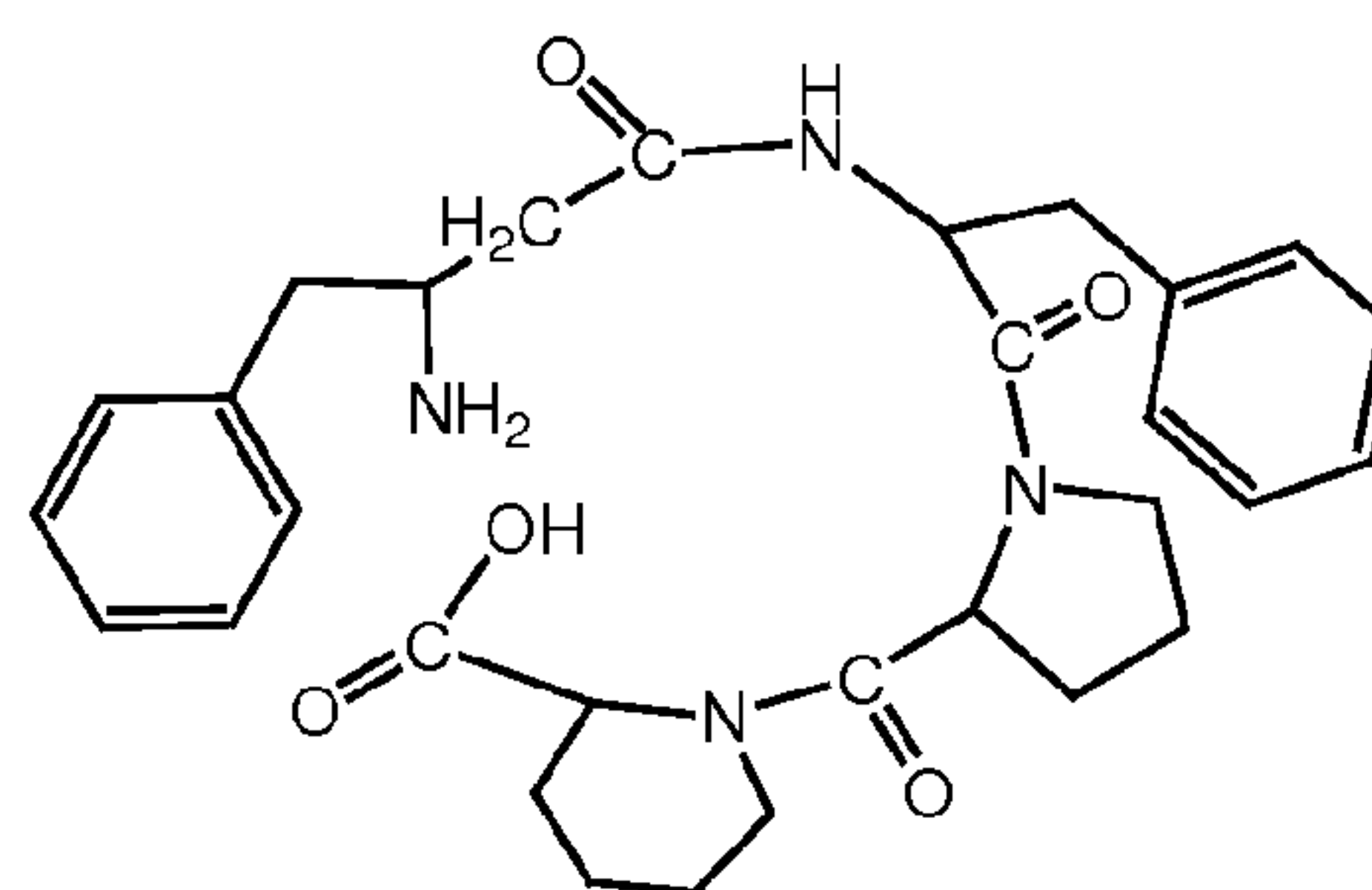
II-3-g (H 2 N- \beta^3 hoPhe-Phe-Pro-Pip-OH),
