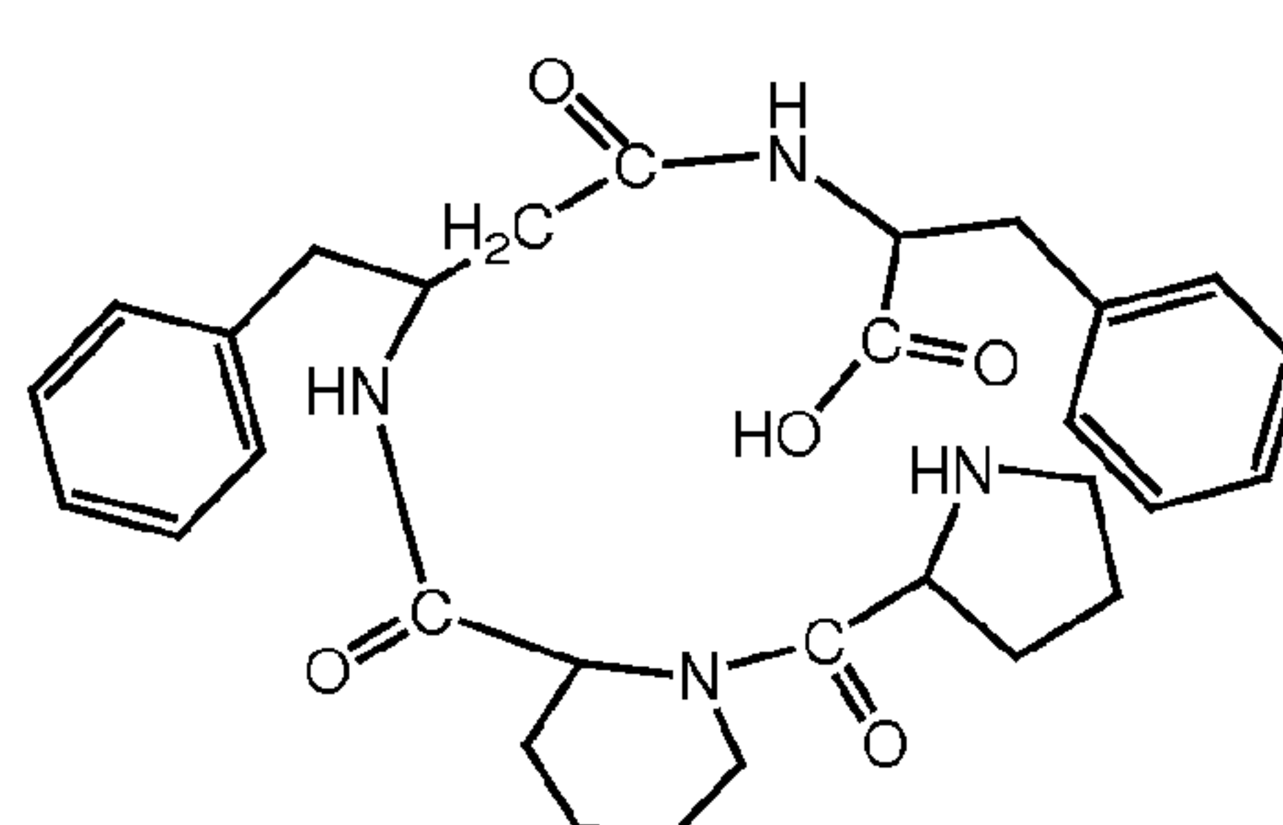
II-3-f (H 2 N- \beta^3 hoPhe-Tyr(t-Bu)-Pro-Pro-OH),
