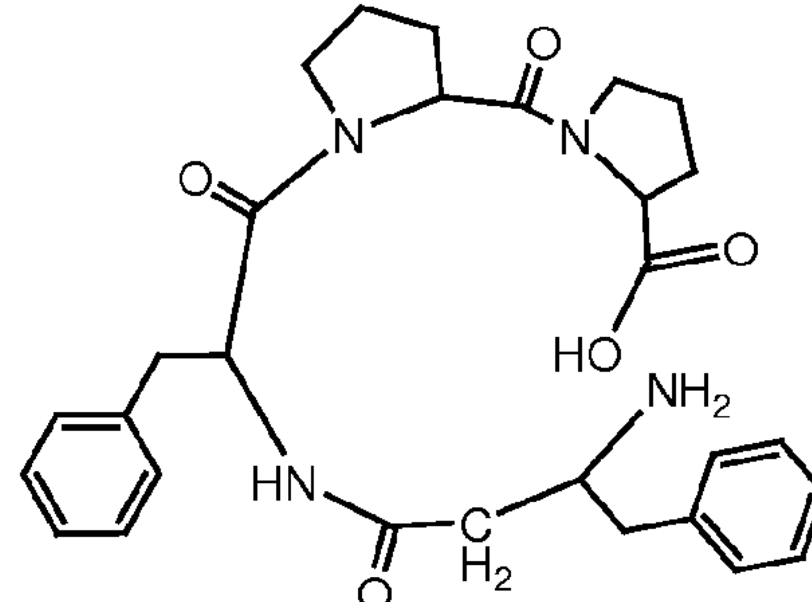
II-3-a (H 2 N-β 3 hoPhe-Phe-Pro-Pro-OH),
