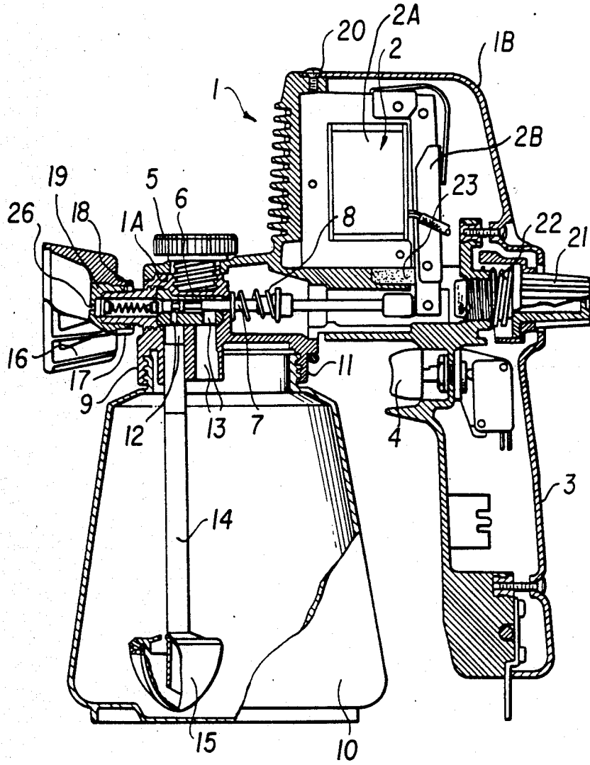
FIG. 9 PRIOR ART
