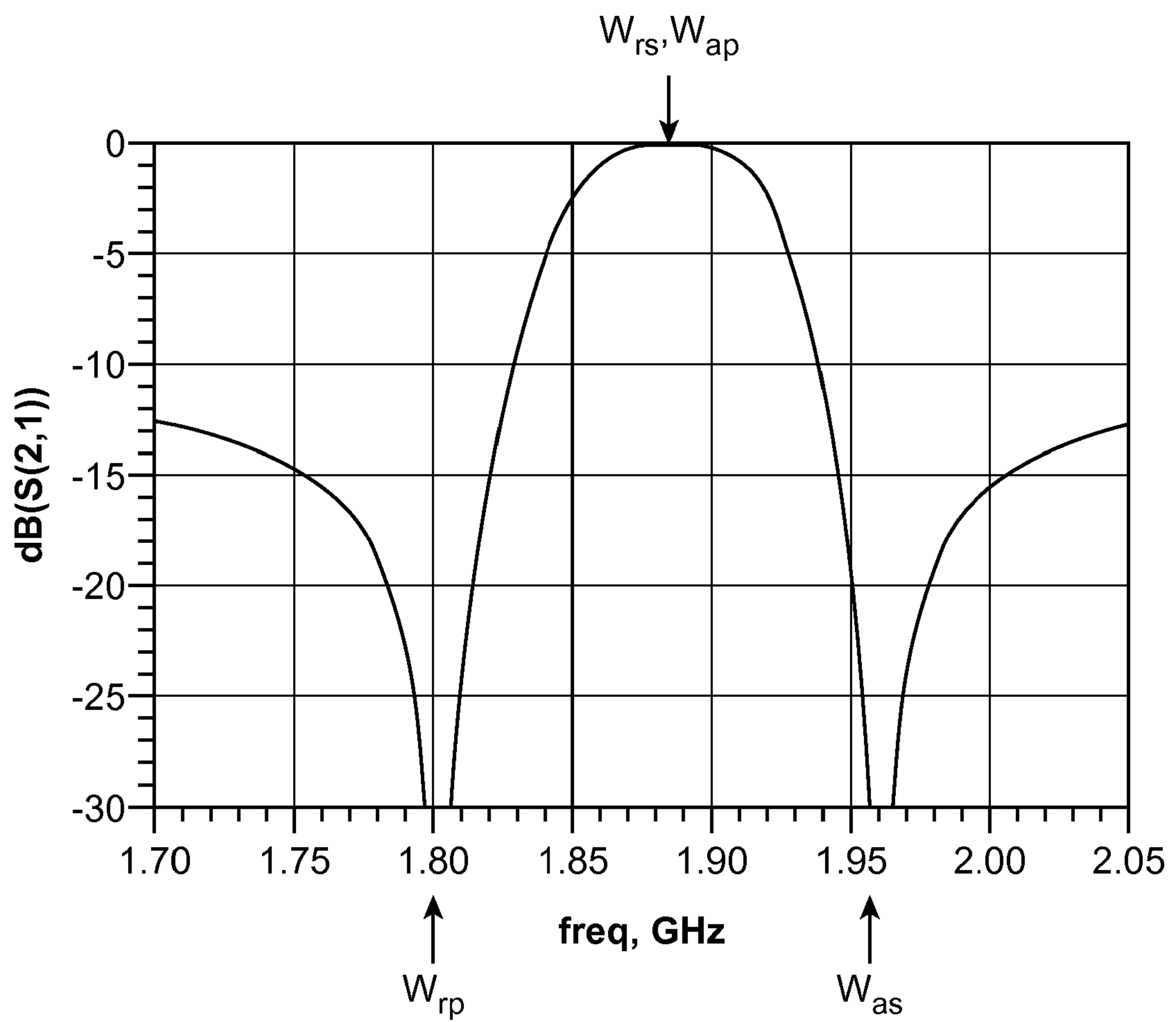
FIG. 3 (PRIOR ART)
