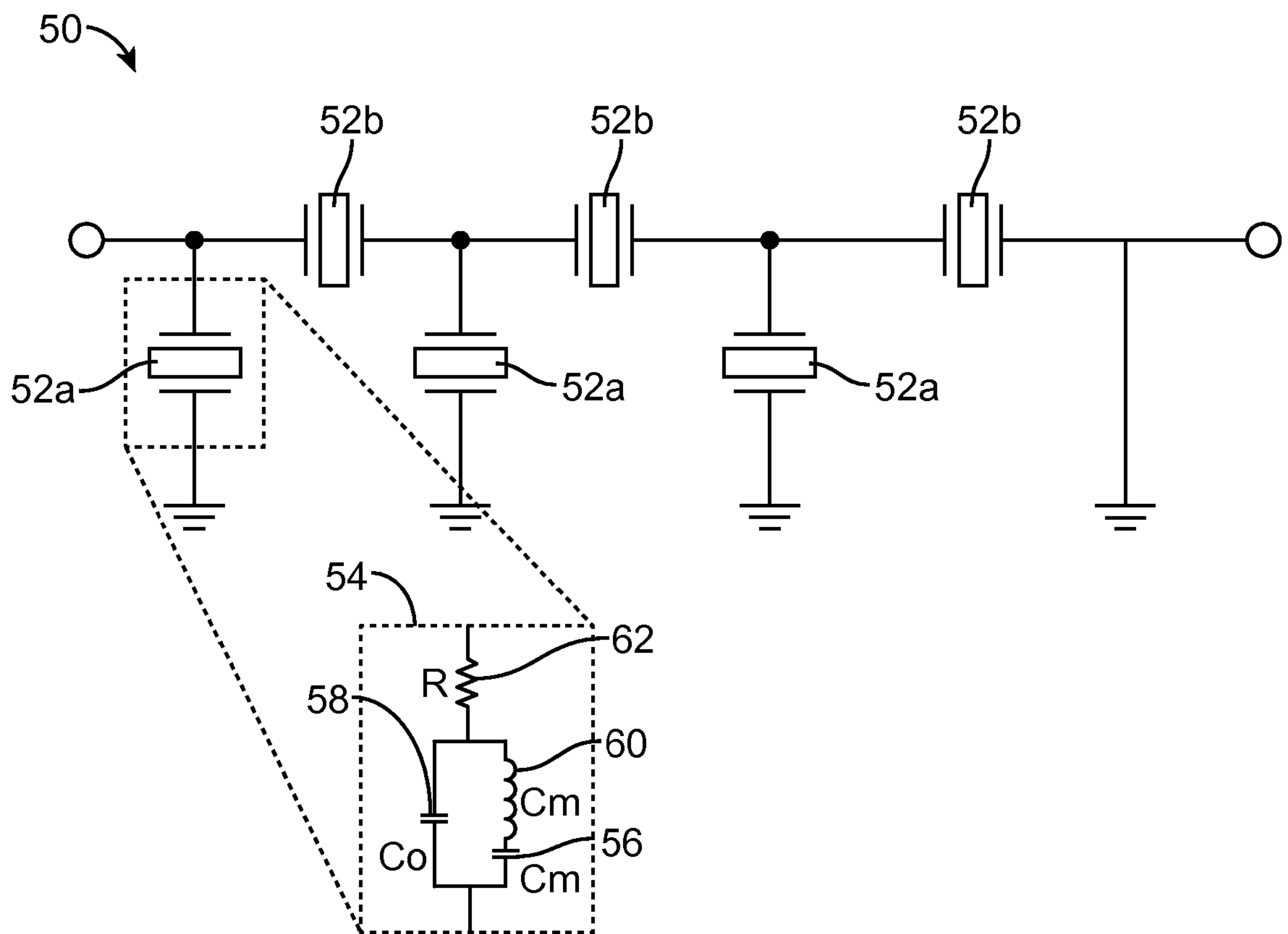
FIG. 2 (PRIOR ART)
