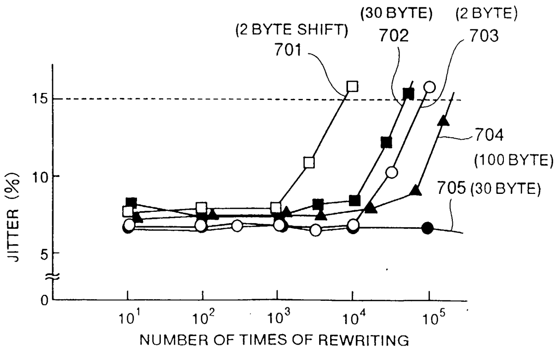
FIG.7 PRIOR ART
