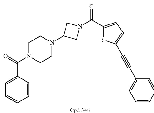
1-(Phenylcarbonyl)-4-(1-{[5-(phenylethynyl)thiophen-2-yl]carbonyl}azetidin-3-yl)piperazine, Cpd 348
