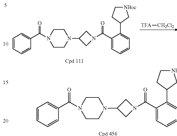
1-(Phenylcarbonyl)-4-{1-[(2-pyrrolidin-3-yl)phenyl]carbonyl]azetidin-3-yl}piperazine, Cpd 456
