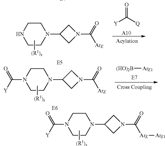
Formula (I)-E
