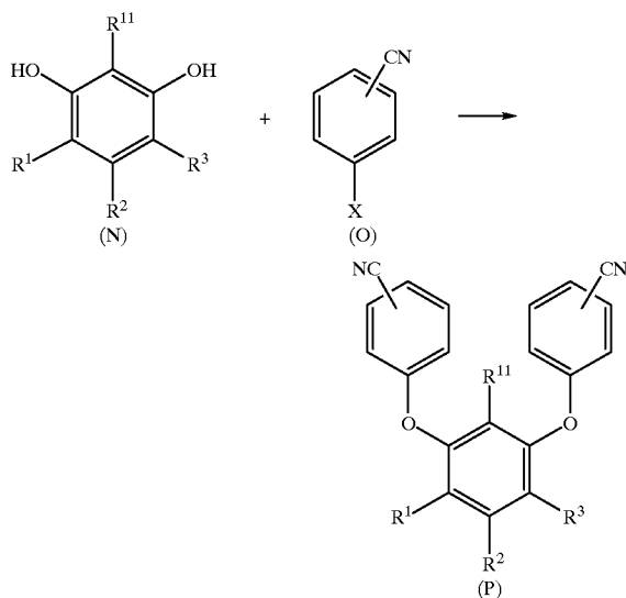
REACTION SCHEME 5
