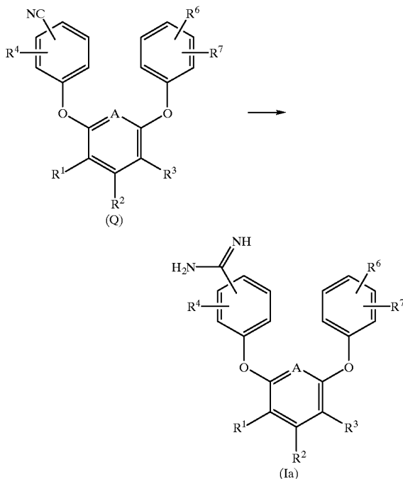
REACTION SCHEME 6
