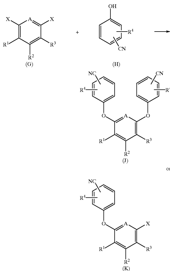
REACTION SCHEME 3
