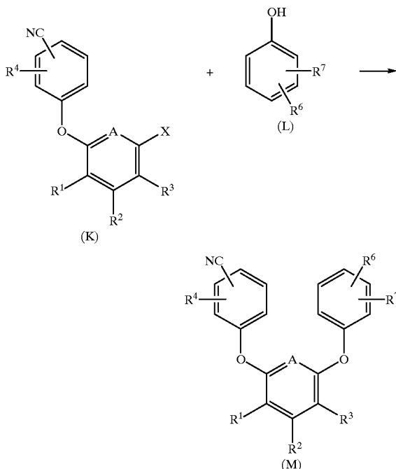
REACTION SCHEME 4
