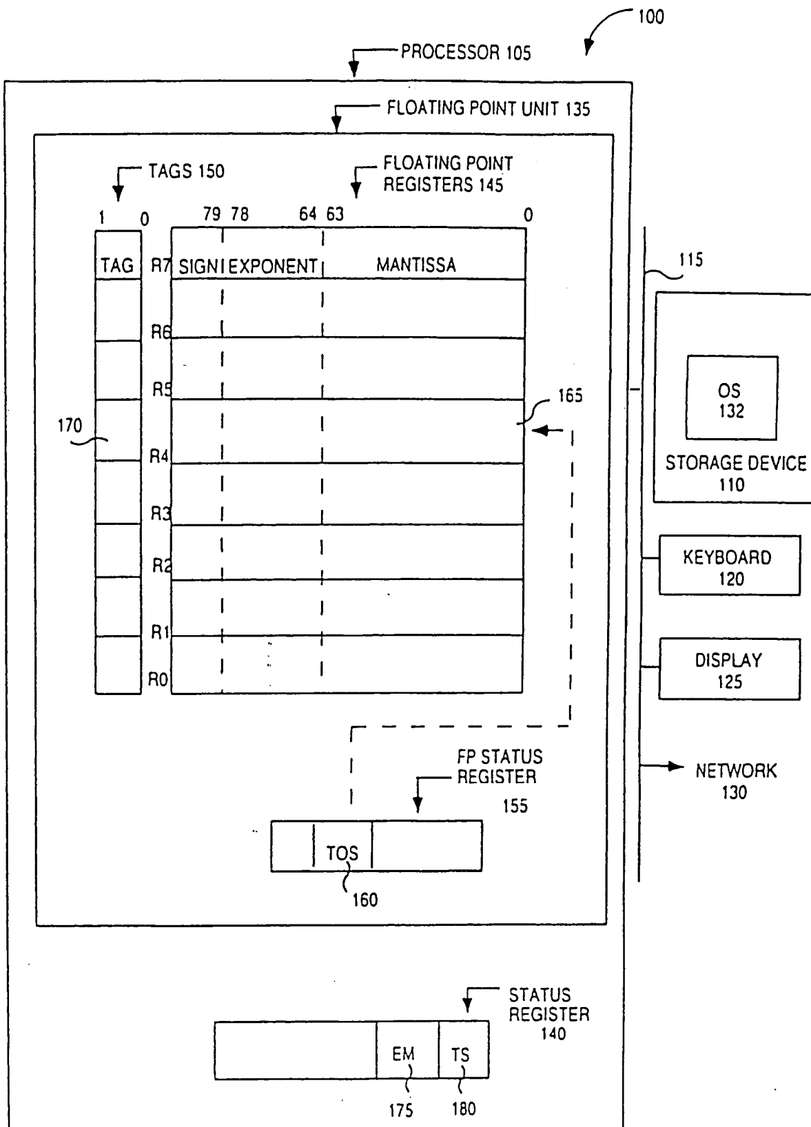
FIG. 1 PRIOR ART
