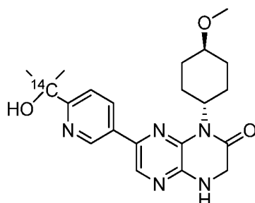
14 C-Compound A
