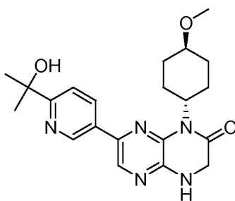
Compound A,
