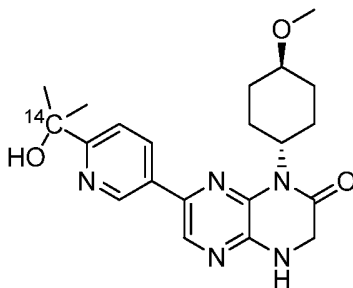
14 C-Compound A
