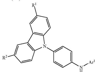
9-(4-aminophenyl) carbazole derivative (Cz2)
