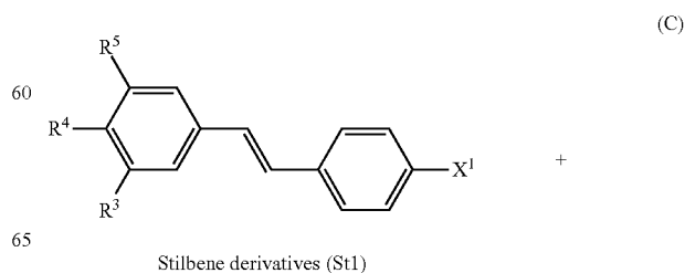
Stilbene derivatives (St1)
