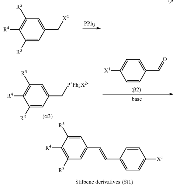
Stilbene derivatives (St1)
