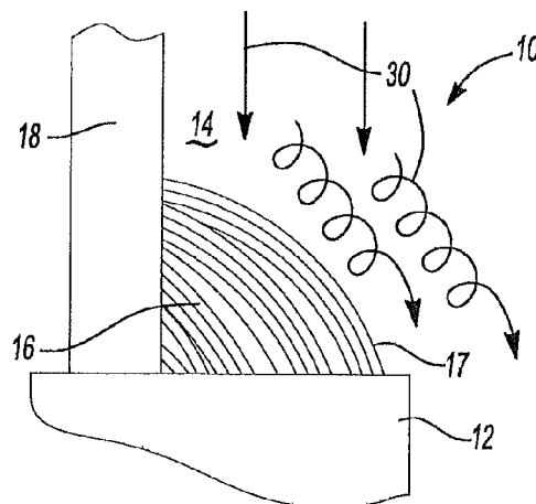
Fig-2 PRIOR ART
