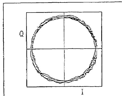
FQPSK-B. VECTOR CONSTELLATION
