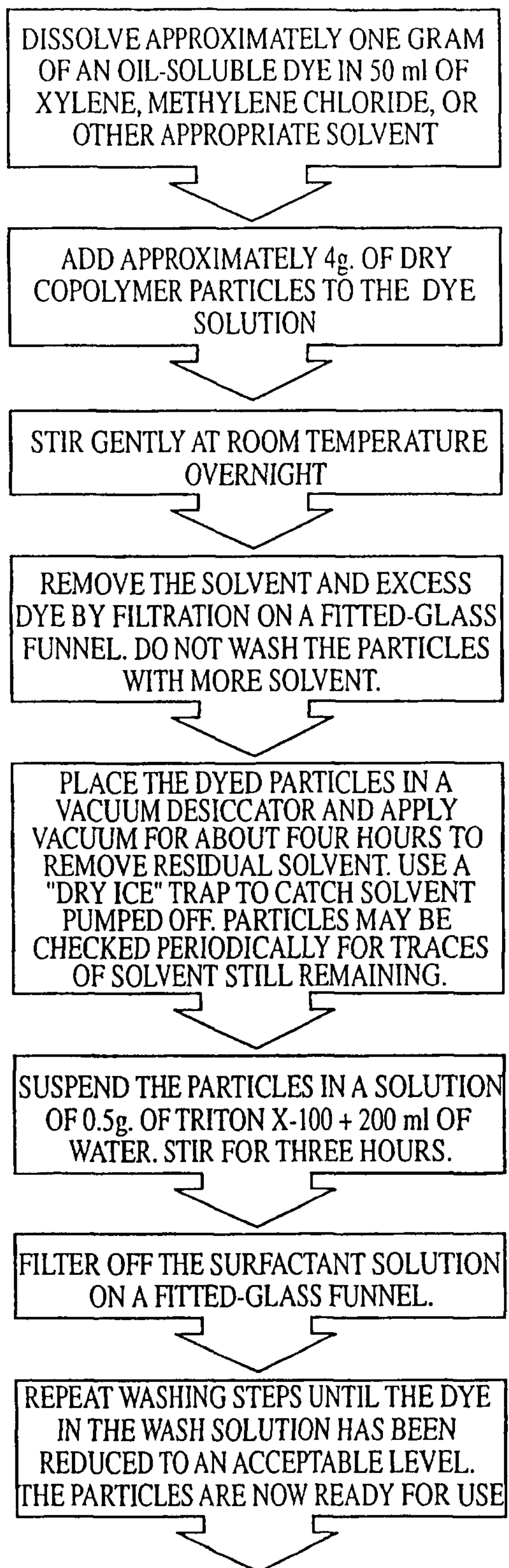
FIG. 1 (PRIOR ART)
