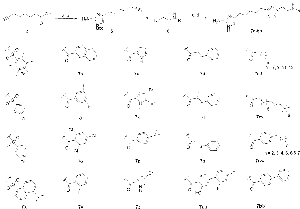
Scheme 2. Synthesis of triazole substituted 2-AI derivatives. a) i. (COCl) 2 , CH 2 Cl 2 , DMF (cat.), ii. CH 2 N 2 , Et 2 O-CH 2 Cl 2 iii. HBr 82 % b) Boc-guanidine, DMF, rt (59 %) c) Azide, CuSO 4 , Na Ascorbate, EtOH, CH 2 Cl 2 , H 2 O d) Trifluoroacetic acid, CH 2 Cl 2 (58 – 94 % over two steps).
