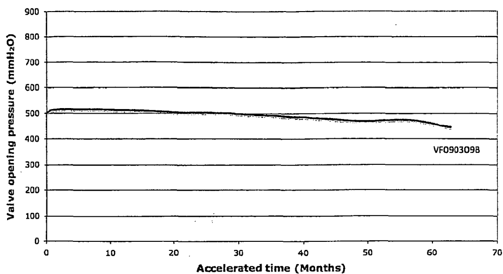
Valve Function stability in Simulated Gastric Fluid
