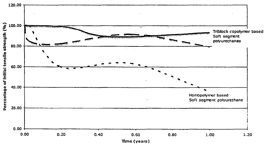
Tensile strength change
