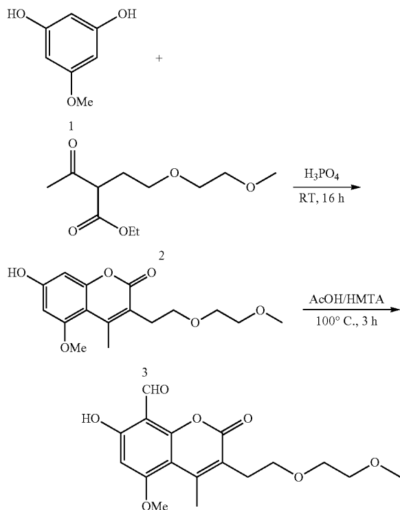
Synthesis of 7-hydroxy-5-methoxy-3-(2-(2-methoxyethoxy)ethyl)-4-methyl-2H-chromene-2-one
