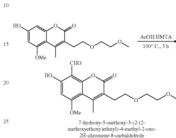
Synthesis of 7-hydroxy-5-methoxy-3-(2-(2-methoxyethoxy)ethyl)-4-methyl-2-oxo-2H-chromene-8-carbaldehyde
