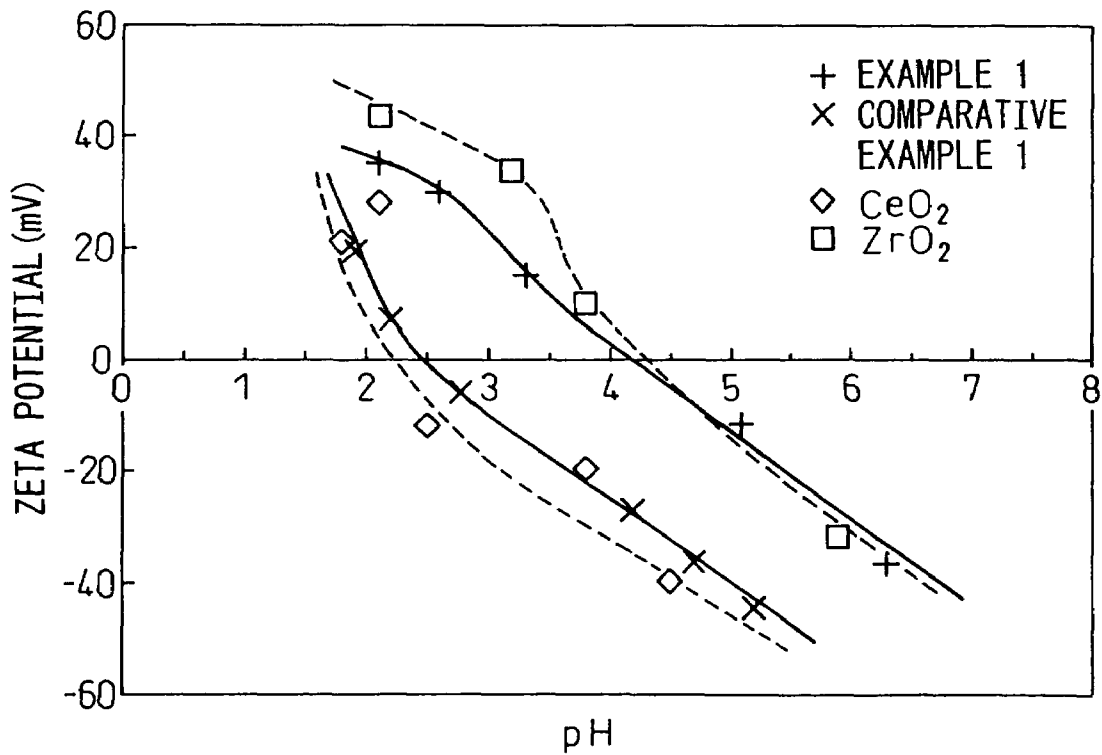
RELATIONSHIP BETWEEN pH AND ZETA POTENTIAL
