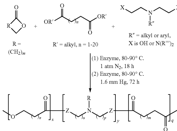
Scheme 1: Preparation of poly(amine-co-ester) terpolymers
