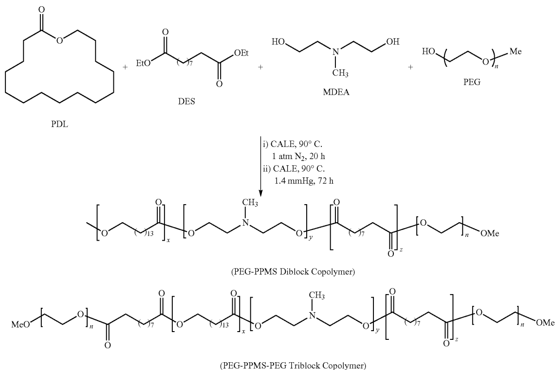
Scheme 2: Enzymatic Synthesis of PEG-PPMS Block Copolymers
