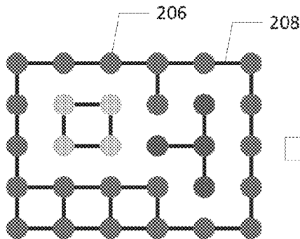
Initial Graph 202
