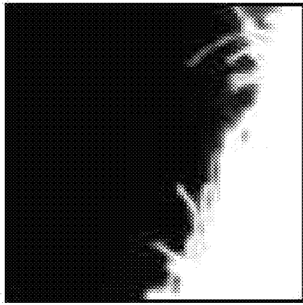
Matting component 806
