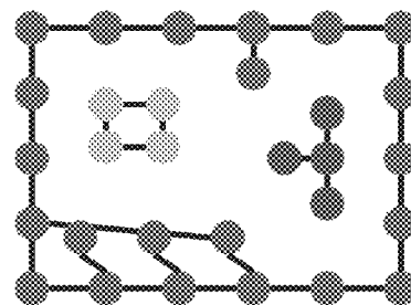
Contracted Graph 204
