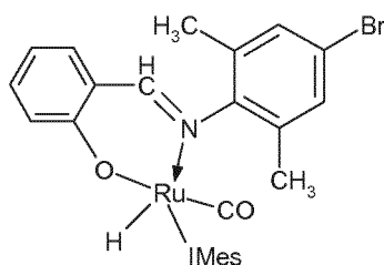
(Ib)-IMes
