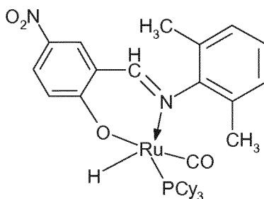
(3c)-PCy 3
