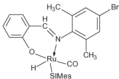
(lb)-SIMes
