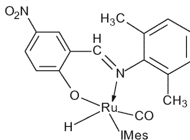
(lc)-IMes
