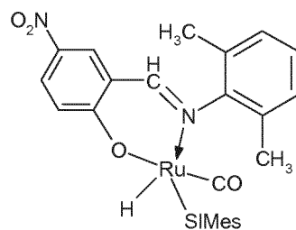
(1c)-SIMes
