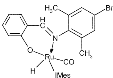
(1b)-IMes
