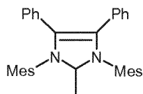
(III d)
