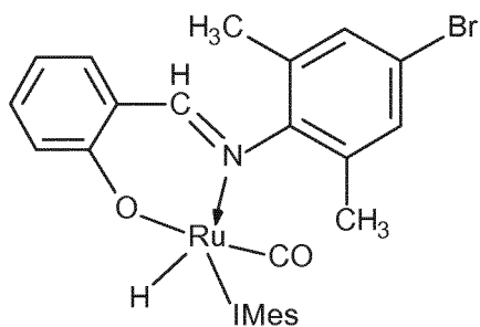
(lb)-IMes
