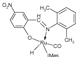
(Ic)-IMes
