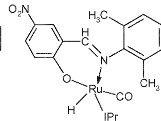
(Ic)-IPr
