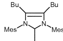
(III f)
