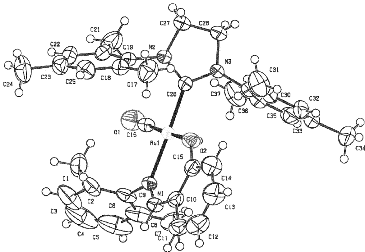
Figure 4: Structure of complex (Ia)-SIMes determined by single crystal XRD analysis
