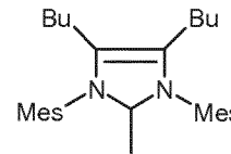
(III f)
