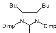
(III t)
