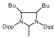
(IIIll)
