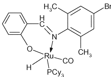
(3b)-PCy 3
