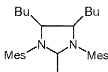
(III e)
