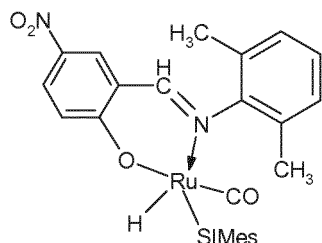
(Ic)-SIMes
