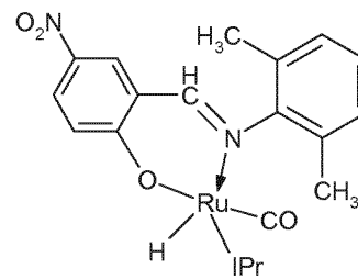
(1c)-IPr
