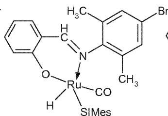
(Ib)-SIMes
