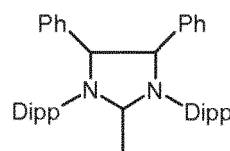
(IIIjj)
