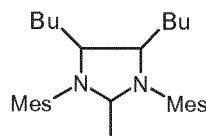
(III e)
