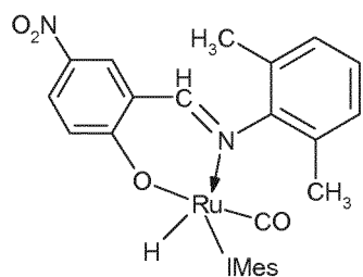
(1c)-IMes
