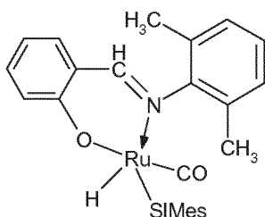
(Ia)-SIMes
