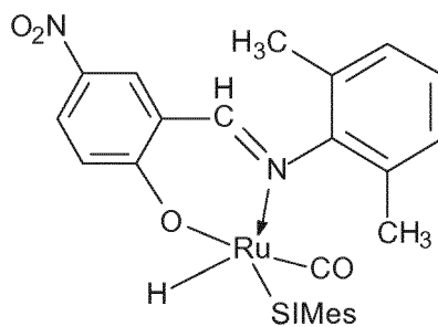
(lc)-SIMes
