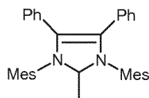
(III d)
