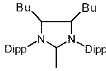
(IIIlm)
