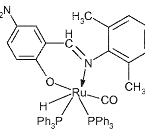
(3c)-PPh 3
