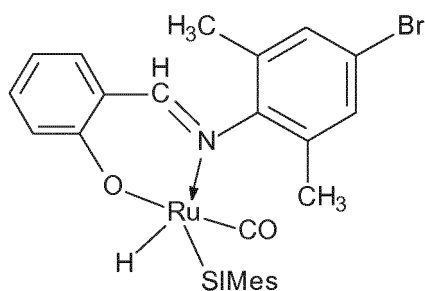
(lb)-SIMes
