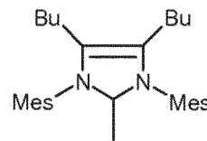
(IIIff)
