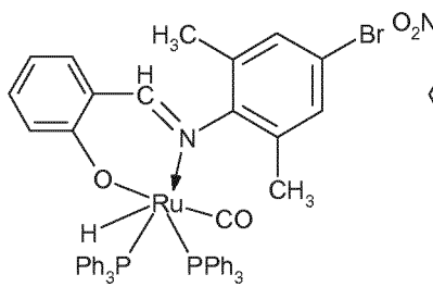
(3b)-PPh 3
