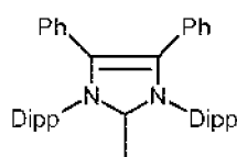
(IIIlk)
