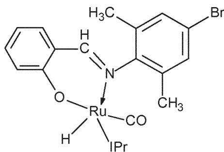
(lb)-IPr
