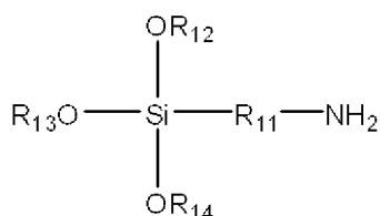
45 Structural Formula (1)
