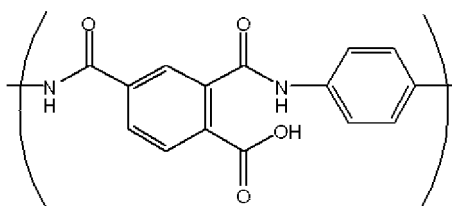
Structural Formula (4)
