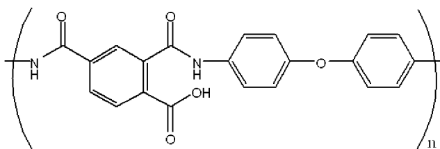
Structural Formula (7)
