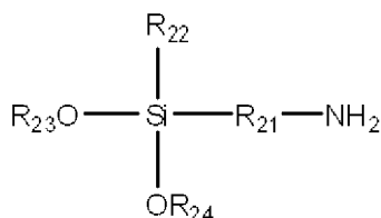
50 Structural Formula (2)
