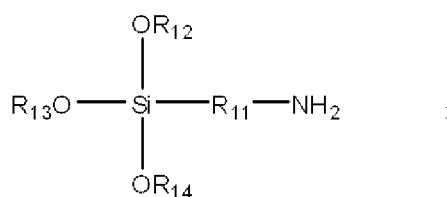
Structural Formula (1)
