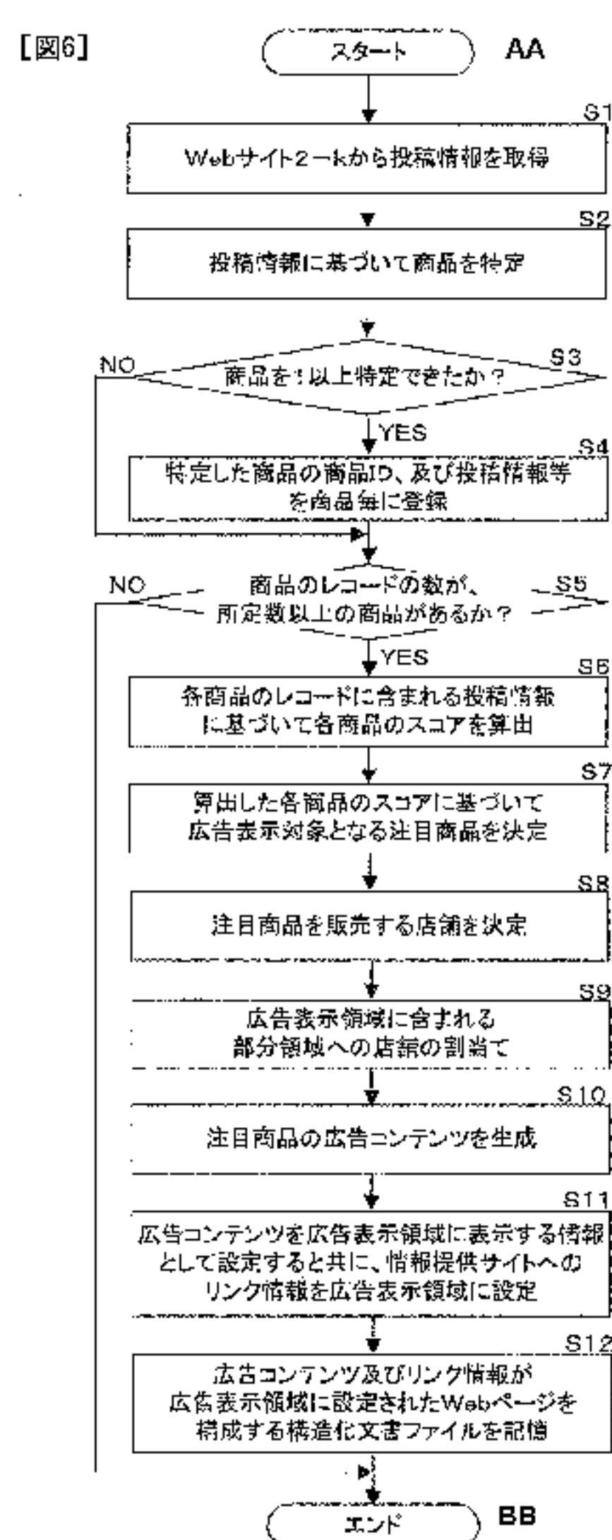
FIG. 6: S1 OBTAIN POSTED INFORMATION FROM WEBSITE (2-K) S2 IDENTIFY PRODUCTS ON BASIS OF POSTED INFORMATION S3 HAVE ONE OR MORE PRODUCTS BEEN IDENTIFIED? S4 FOR EACH PRODUCT, REGISTER PRODUCT ID OF IDENTIFIED PRODUCT, POSTED INFORMATION, ETC. S5 DOES NUMBER OF PRODUCT RECORDS INCLUDE AT LEAST PRESCRIBED NUMBER OF PRODUCTS? S6 CALCULATE SCORE FOR EACH PRODUCT ON BASIS OF POSTED INFORMATION INCLUDED IN EACH PRODUCT RECORD S7 DETERMINE FEATURED PRODUCT TO BE DISPLAYED IN ADVERTISEMENT ON BASIS OF CALCULATED SCORE FOR EACH PRODUCT S8 DETERMINE STORES SELLING FEATURED PRODUCT S9 ALLOCATE STORES TO PARTIAL REGIONS INCLUDED IN ADVERTISEMENT DISPLAY REGION S10 GENERATE ADVERTISEMENT CONTENT FOR FEATURED PRODUCT S11 SET ADVERTISEMENT CONTENT AS INFORMATION TO BE DISPLAYED IN ADVERTISEMENT DISPLAY REGION, AND SET LINK INFORMATION FOR INFORMATION-PROVIDING WEBSITE IN ADVERTISEMENT DISPLAY REGION S12 STORE STRUCTURED DOCUMENT FILE THAT CONFIGURES WEB PAGE ON WHICH ADVERTISEMENT CONTENT AND LINK INFORMATION IS SET IN ADVERTISEMENT DISPLAY REGION AA START BB END
