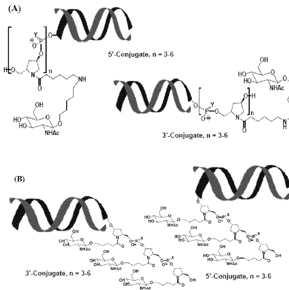
Figure 25. GalNAc custers for hepatic targeting
