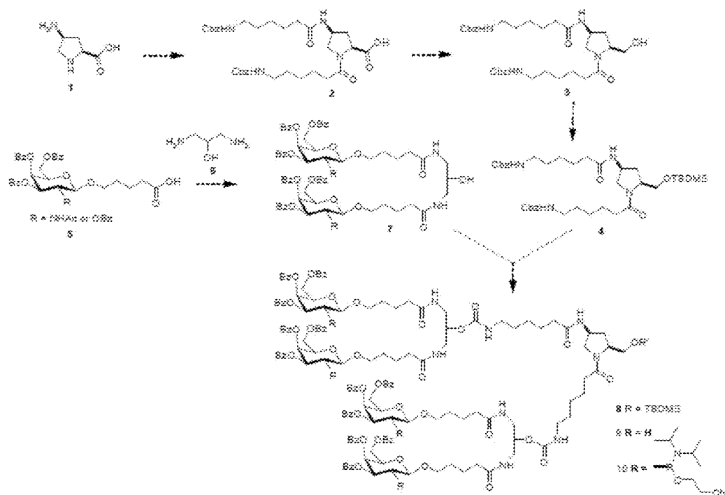
Figure 29. Synthesis of Mannose conjugate building blocks
