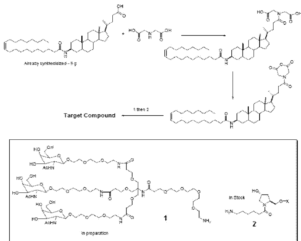
Figure 21. Glycolipid-siRNA Conjugate: Synthesis
