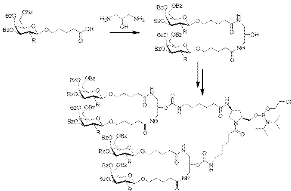
Figure 26. Carbohydrate (GalNAC) clusters for conjugation to siRNA
