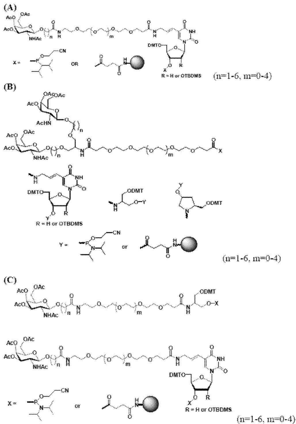
Figure 22. Monomers for carbohydrate conjugation to siRNA
