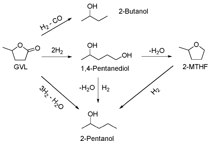
Scheme 1. Selective hydrogenation products from GVL.
