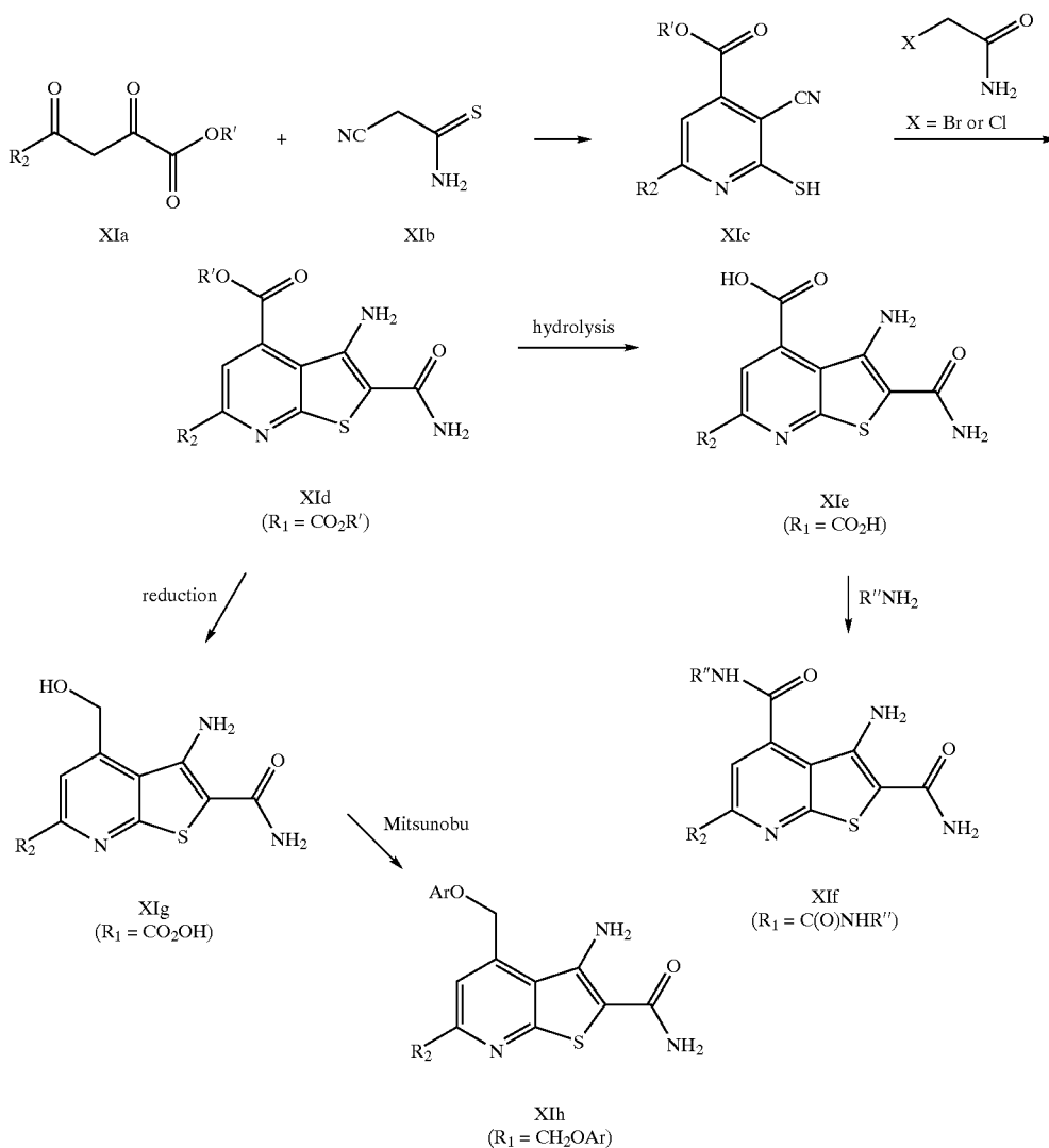
Scheme XI
