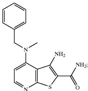
3-Amino-4-(methyl-phenethyl-amino)-thieno[2,3-b] pyridine-2-carboxylic acid amide
