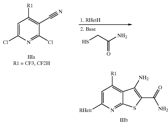
Scheme III
