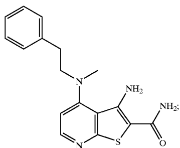
3-Amino-4-(4-benzyl-piperidin-1-yl)-thieno[2,3-b] pyridine-2-carboxylic acid amide
