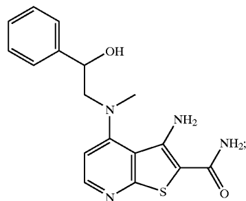
4-(3-Amino-2-carbamoyl-thieno[2,3-b]pyridin-4-yl)- piperazine-1-carboxylic acid benzyl ester
