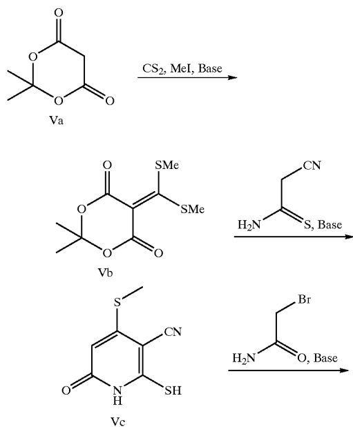
Scheme V
