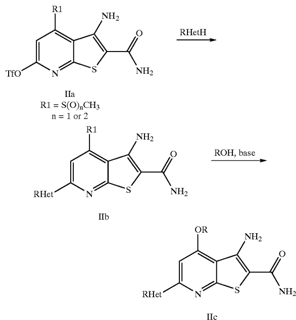
Scheme II
