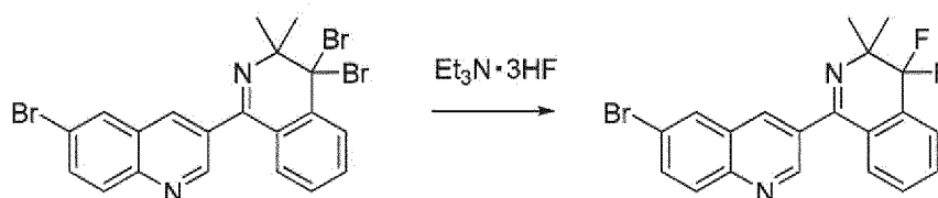
[Chemical Formula 13]
