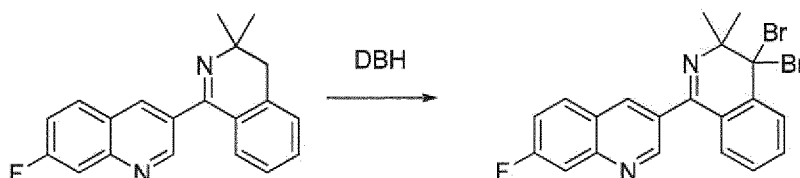
[Chemical Formula 15]
