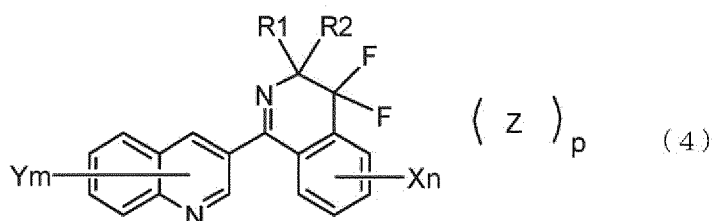
[Chemical Formula 6]
