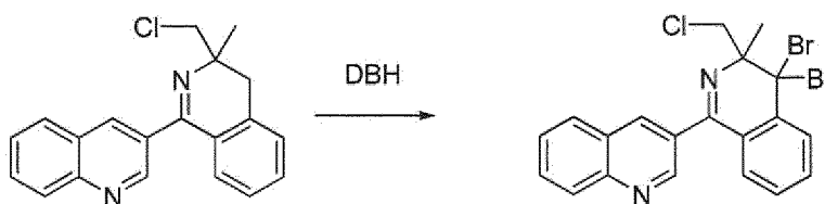
[Chemical Formula 17]
