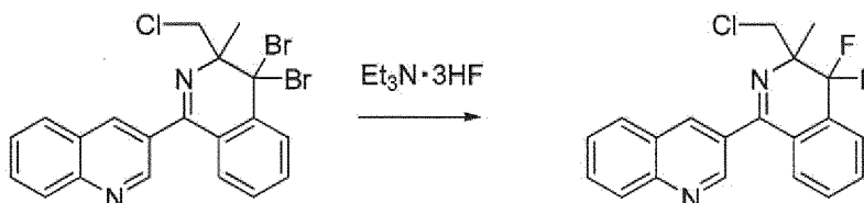
[Chemical Formula 18]
