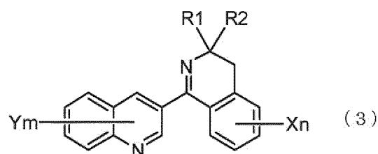
[Chemical Formula 5]
