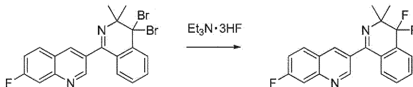
[Chemical Formula 16]
