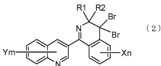
[Chemical Formula 21]
