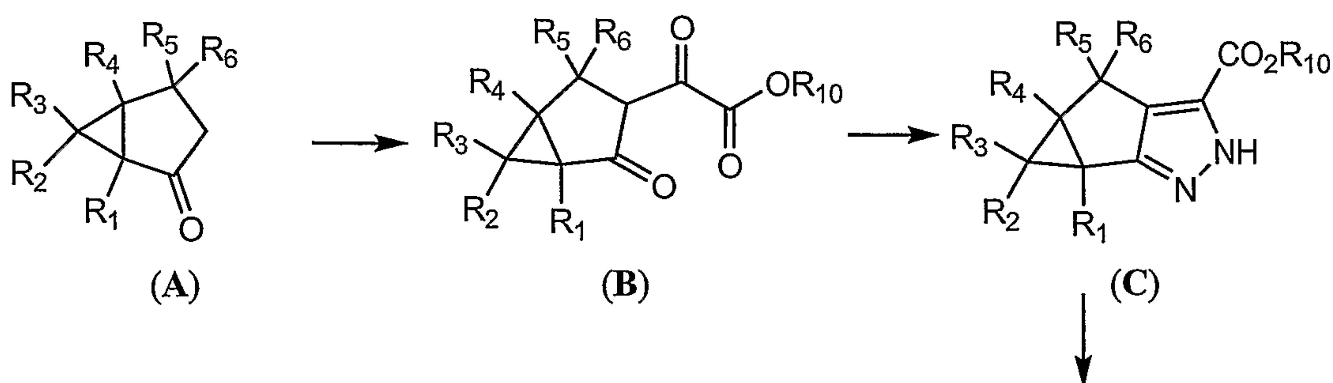
Scheme I
