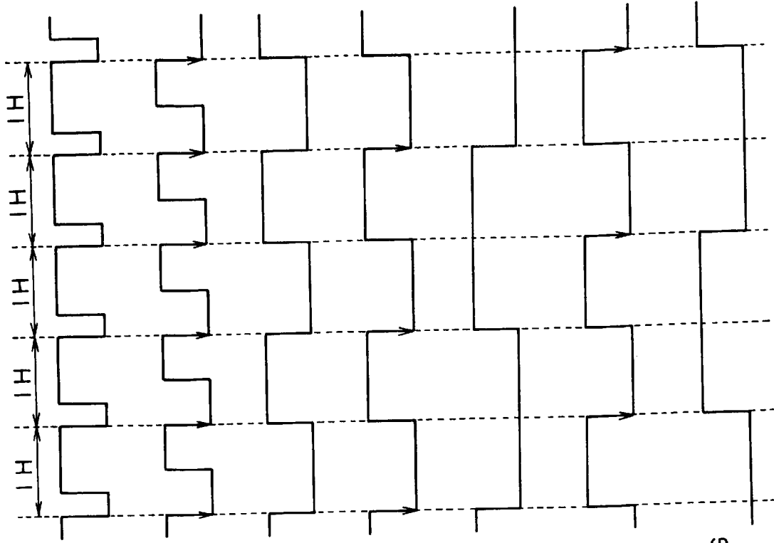
INVERSE TIMING SIGNAL HT3
