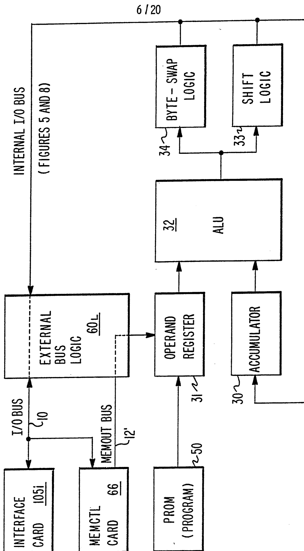
FIG. 5. Data Manipulation Logic Block Diagram.
