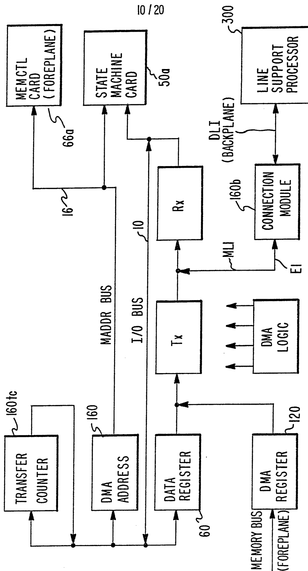
FIG. 9. MLI Interface Block Diagram.
