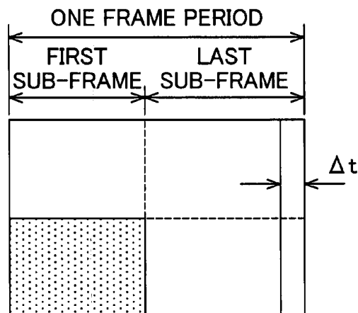
(TWO-PART DIVISION, LUMINANCE 1/4)
