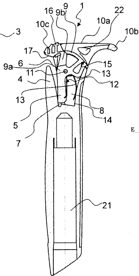
FIG. 14 Section E-E
