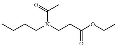
ethyl 3-(N-butylacetamino)propionate
