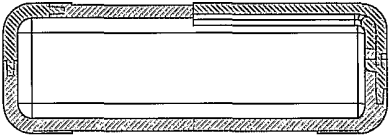
FIG 37 SECTION F - F
