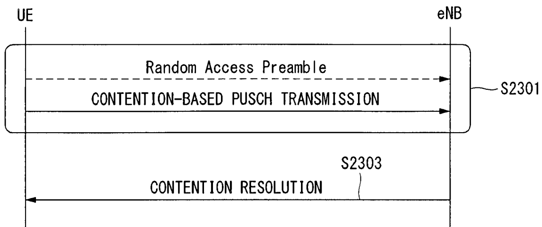
(a) CONTENTION-BASED RANDOM ACCESS PROCEDURE
