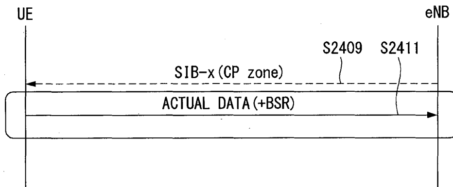
(b) UL RESOURCE ALLOCATION PROCEDURE OF 1 STEP
