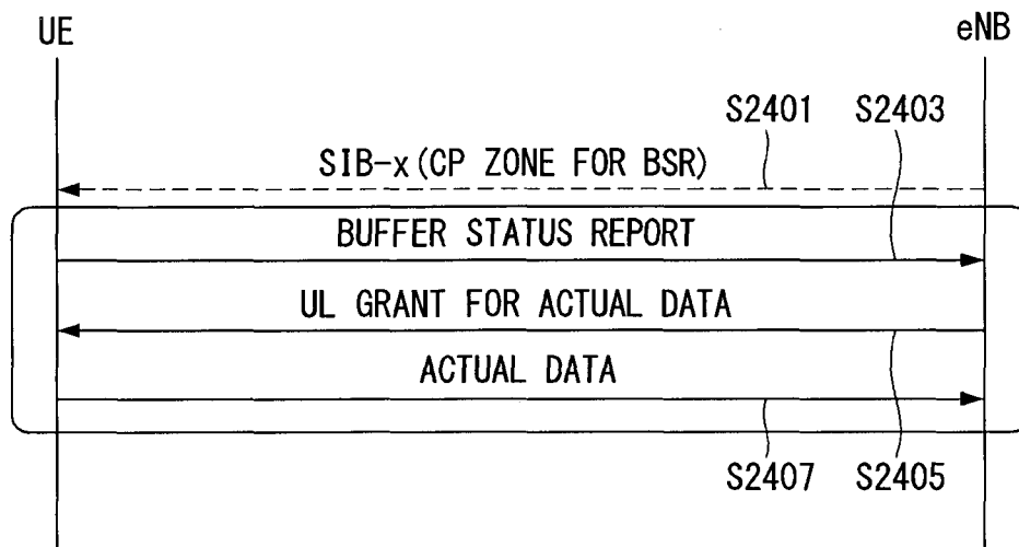
(a) UL RESOURCE ALLOCATION PROCEDURE OF 3 STEPS
