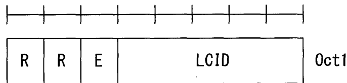
R/R/E/LCID sub-header
