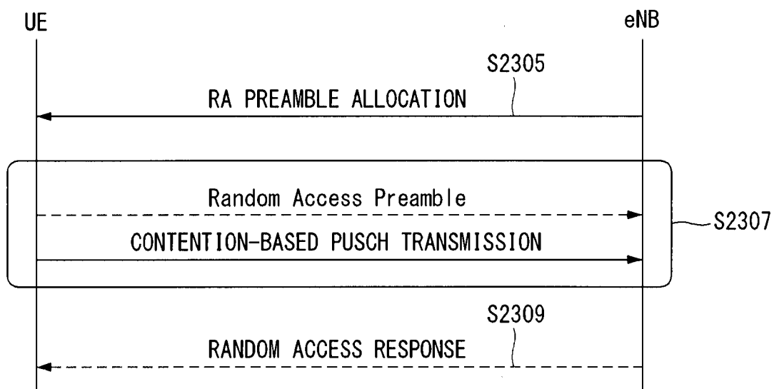
(b) NON-CONTENTION-BASED RANDOM ACCESS PROCEDURE
