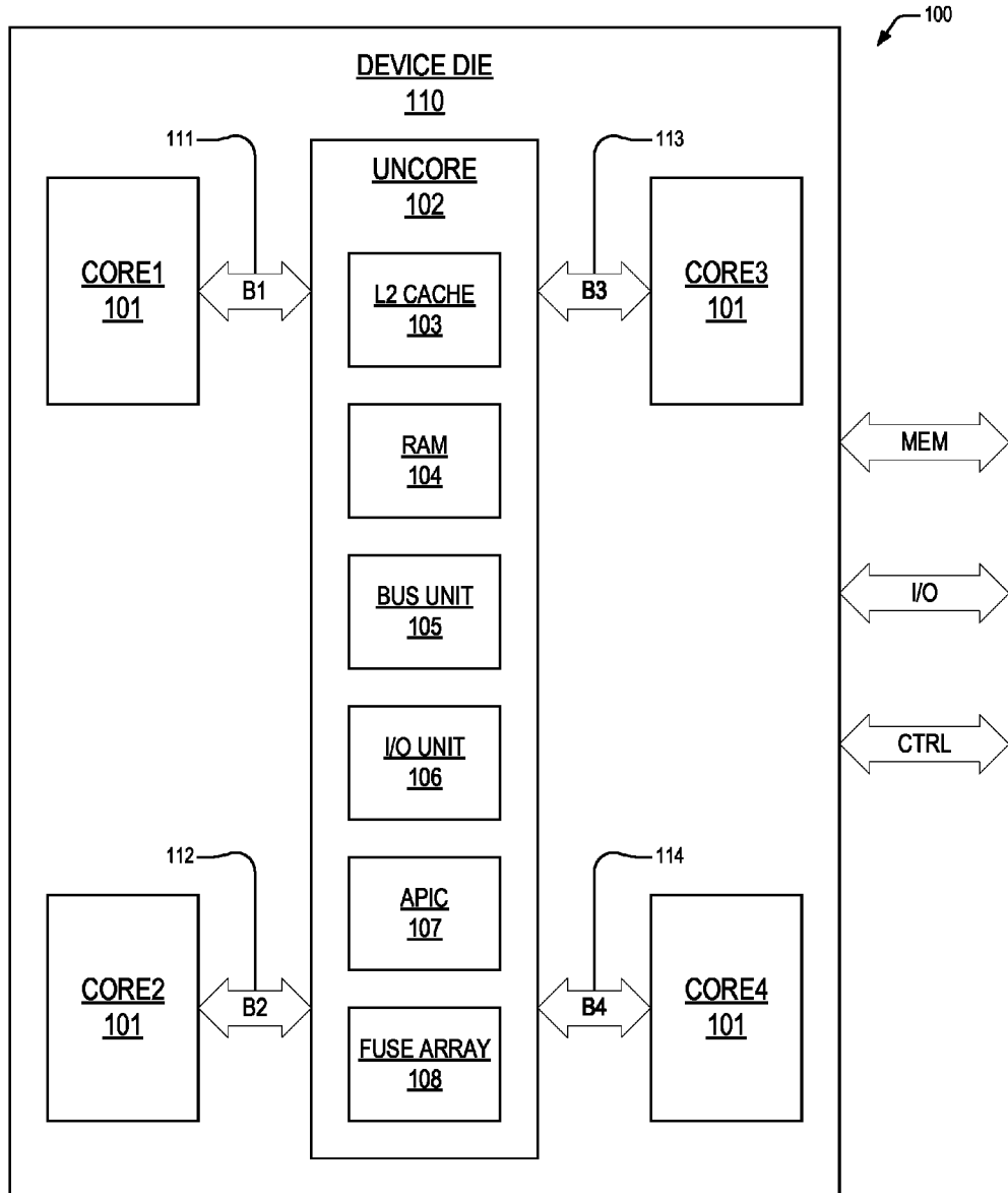
FIG. 1 (Prior Art) MULTI-CORE PROCESSOR WITH NON-CORE COMMON RESOURCES
