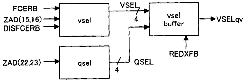
FIG. 7 Vertical Block Select Signal Buffer Circuit
