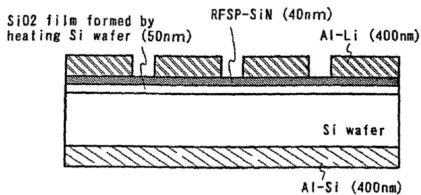
Fig. 29B MOS structure comprising RFSP-SiN film
