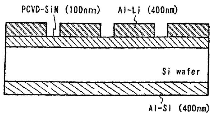
Fig. 29A MOS structure comprising PCVD-SiN film
