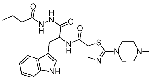
N -(1-(2-butyrylhydrazinyl)-3-(1 H -indol-3-yl)-1-oxopropan-2-yl)-2-(4-methylpiperazin-1-yl)thiazole-5-carboxamide;
