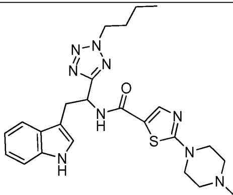
N -(1-(2-butyl-2 H -tetrazol-5-yl)-2-(1 H -indol-3-yl)ethyl)-2-(4-methylpiperazin-1-
