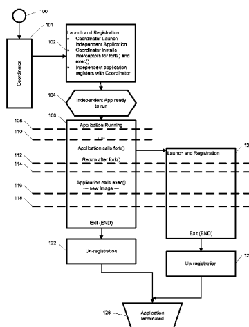
Incremental checkpointing of application groups using a mix of exec and fork/kill
