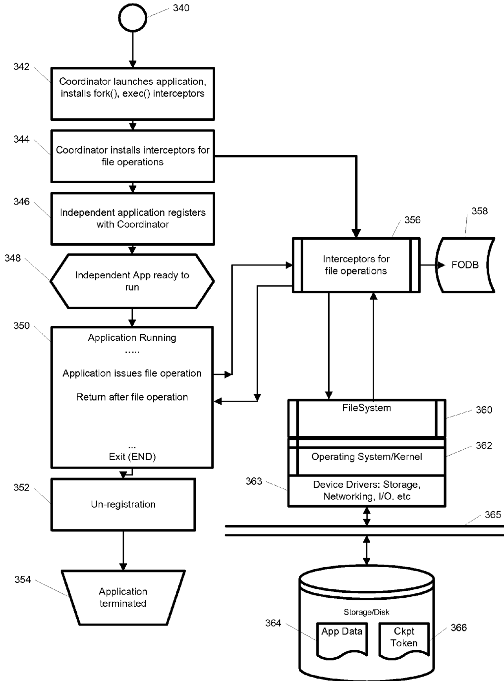
Fig. 12 File Operations logging
