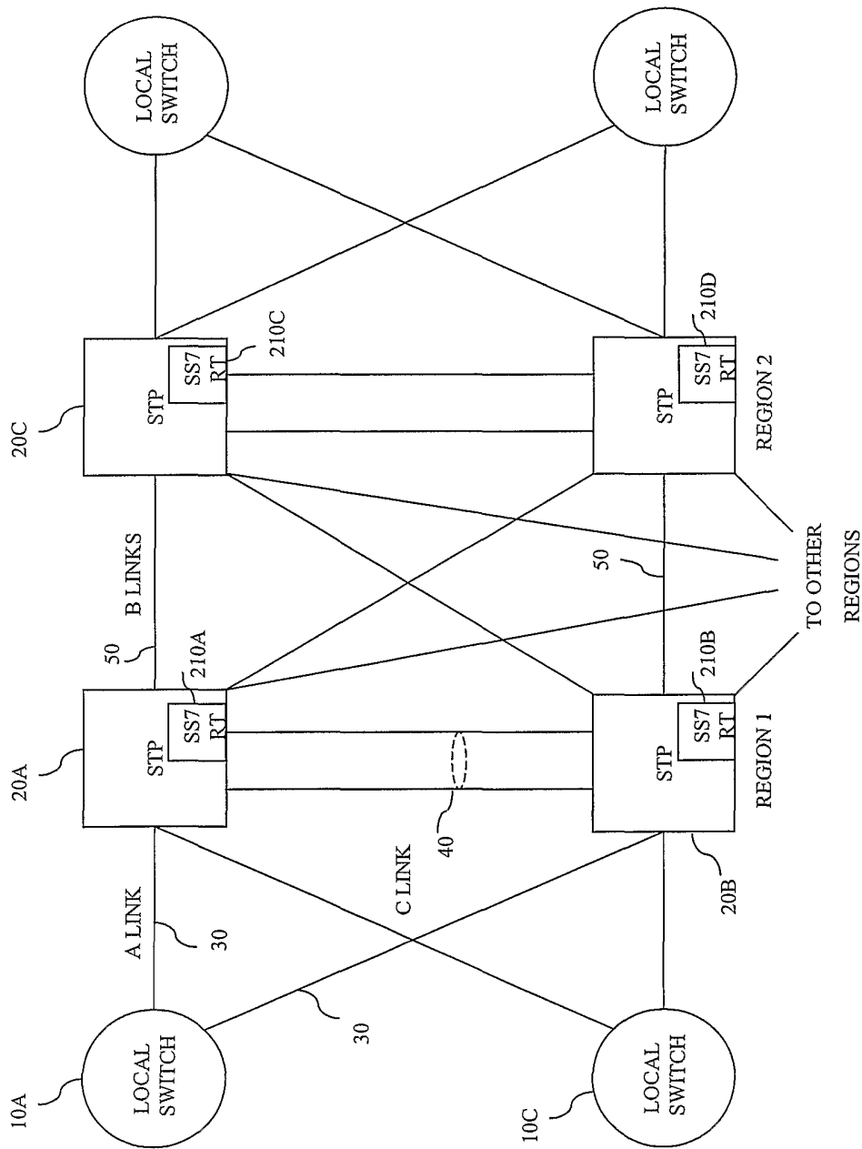
FIGURE 2 (PRIOR ART)
