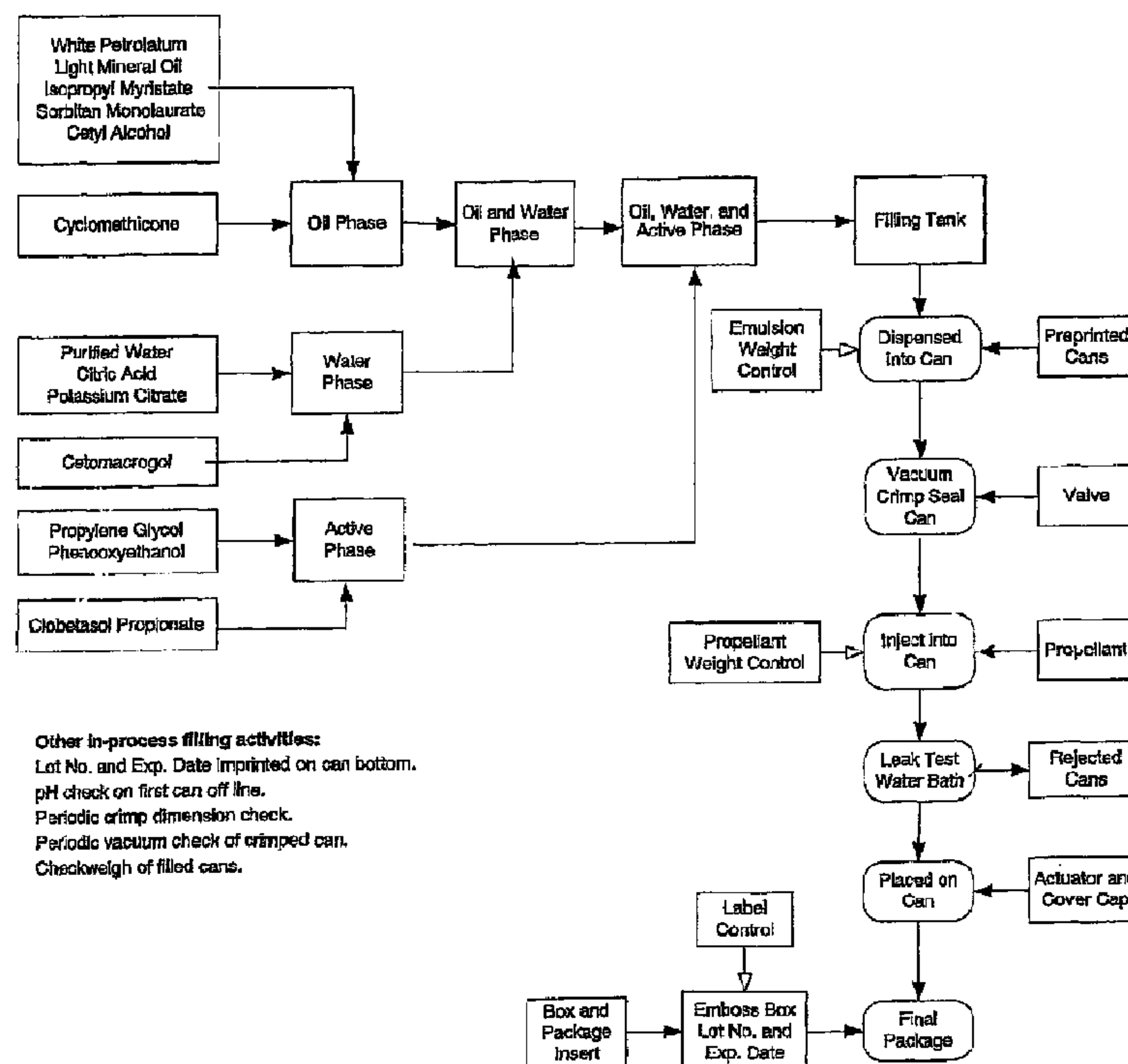
Ethanol-Free Clobetasol Propionate Foam, 0.05% Process Flow Diagram
