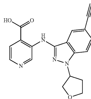
3-{[5-ethynyl-1-(tetrahydrofuran-3-yl)-1H-indazol-3-yl]amino}pyridine-4-carboxylic acid
