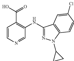
3-{5-chloro-(1-cyclopropyl-1H-indazol-3-yl)amino}pyridine-4-carboxylic acid
