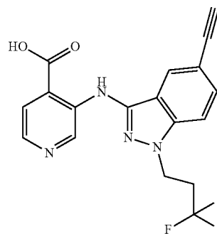
3-{[5-ethynyl-1-(3,3,3-trifluoropropyl)-1H-indazol-3-yl]amino}pyridine-4-carboxylic acid
