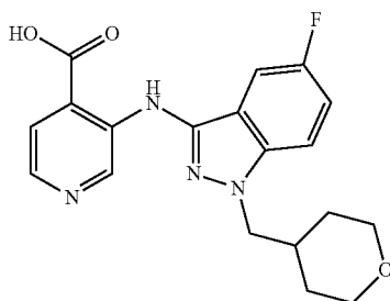
3-{[5-fluoro-1-(tetrahydro-2H-pyran-4-ylmethyl)-1H-indazol-3-yl]amino}pyridine-4-carboxylic acid
