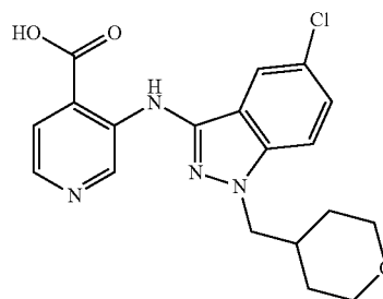
3-{[5-chloro-1-(tetrahydro-2H-pyran-4-ylmethyl)-1H-indazol-3-yl]amino}pyridine-4-carboxylic acid
