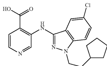
3-{[1-(2-cyclopentylethyl)-5-fluoro-1H-indazol-3-yl]amino}pyridine-4-carboxylic acid
